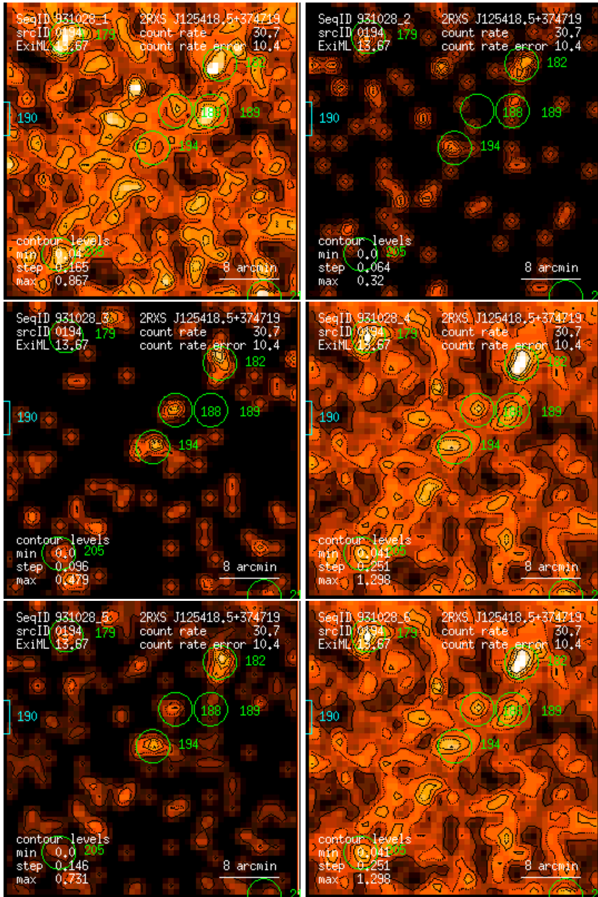
Figure 194: RASS 931028: detection 0194: band rate images, Gaussian filter: (1) PSPC channels 11 – 41, (2) 52 – 90, (3) 91 – 201, (4) 11 – 235, (5) 52 – 201, (6) 11 – 201. Broad band rates in counts/ks. Band rate contour levels in counts/ks/arcmin 2 .
