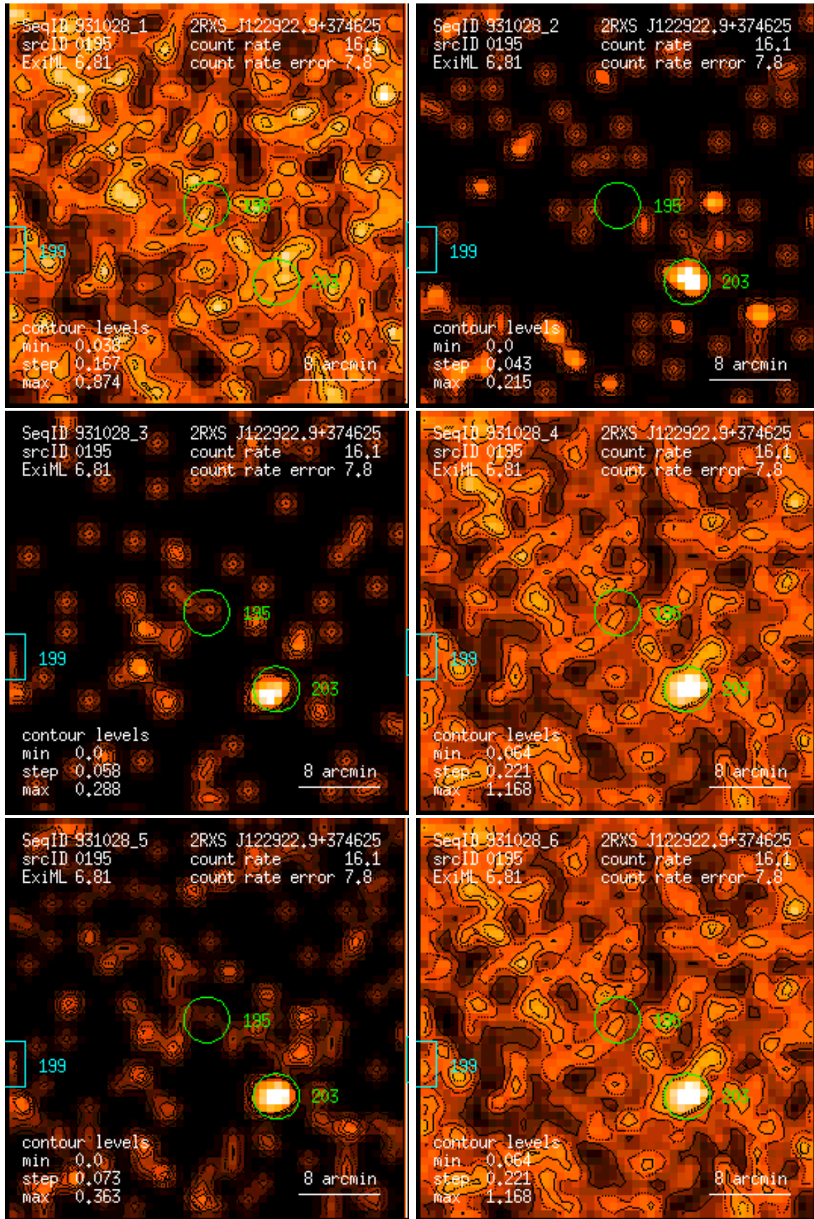
Figure 195: RASS 931028: detection 0195: band rate images, Gaussian filter: (1) PSPC channels 11 – 41, (2) 52 – 90, (3) 91 – 201, (4) 11 – 235, (5) 52 – 201, (6) 11 – 201. Broad band rates in counts/ks. Band rate contour levels in counts/ks/arcmin 2 .
