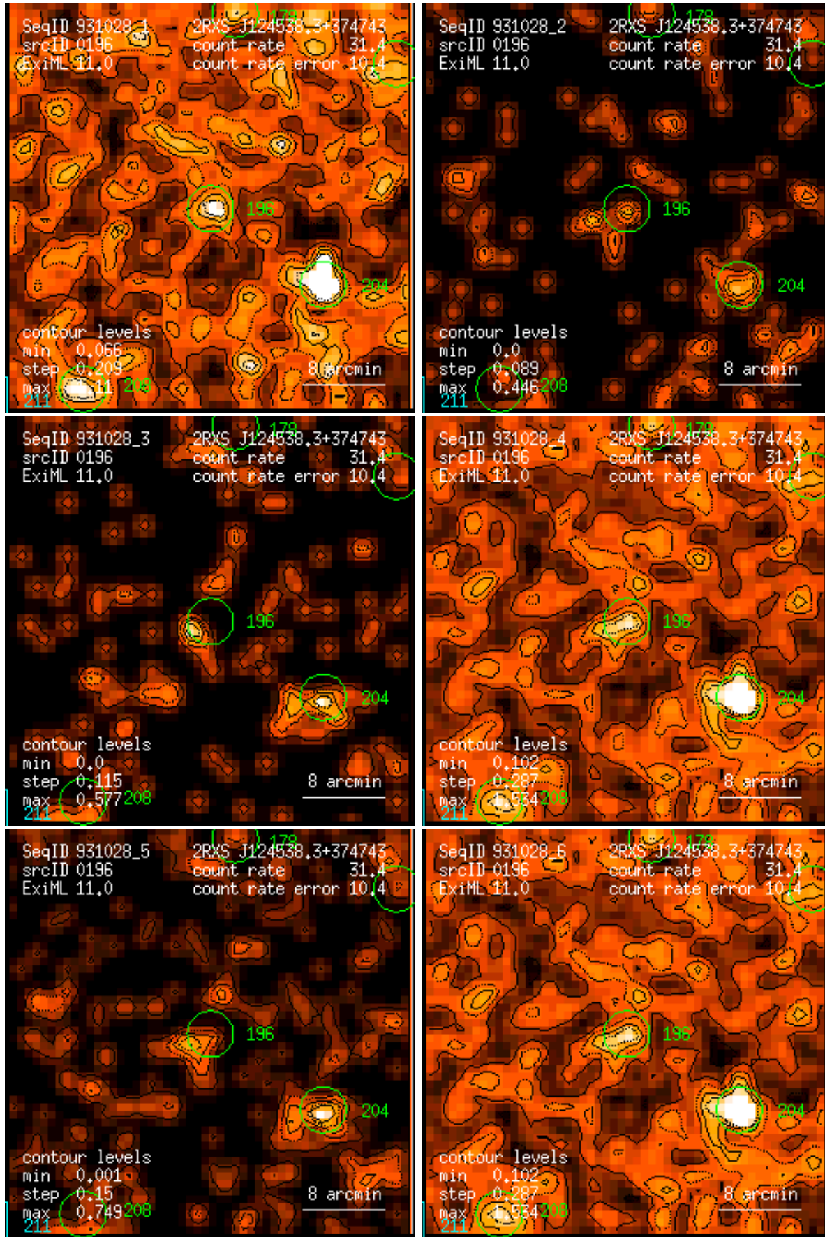
Figure 196: RASS 931028: detection 0196: band rate images, Gaussian filter: (1) PSPC channels 11 – 41, (2) 52 – 90, (3) 91 – 201, (4) 11 – 235, (5) 52 – 201, (6) 11 – 201. Broad band rates in counts/ks. Band rate contour levels in counts/ks/arcmin 2 .
