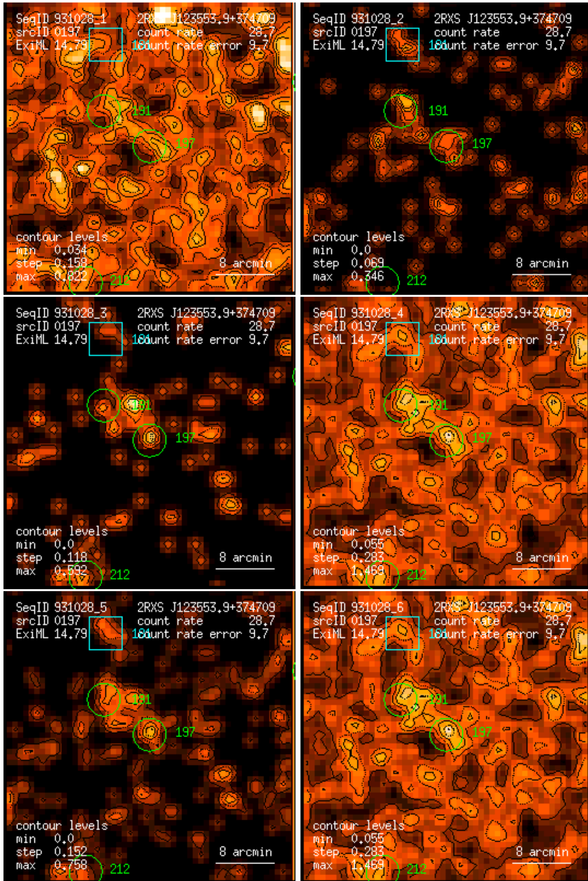
Figure 197: RASS 931028: detection 0197: band rate images, Gaussian filter: (1) PSPC channels 11 – 41, (2) 52 – 90, (3) 91 – 201, (4) 11 – 235, (5) 52 – 201, (6) 11 – 201. Broad band rates in counts/ks. Band rate contour levels in counts/ks/arcmin 2 .
