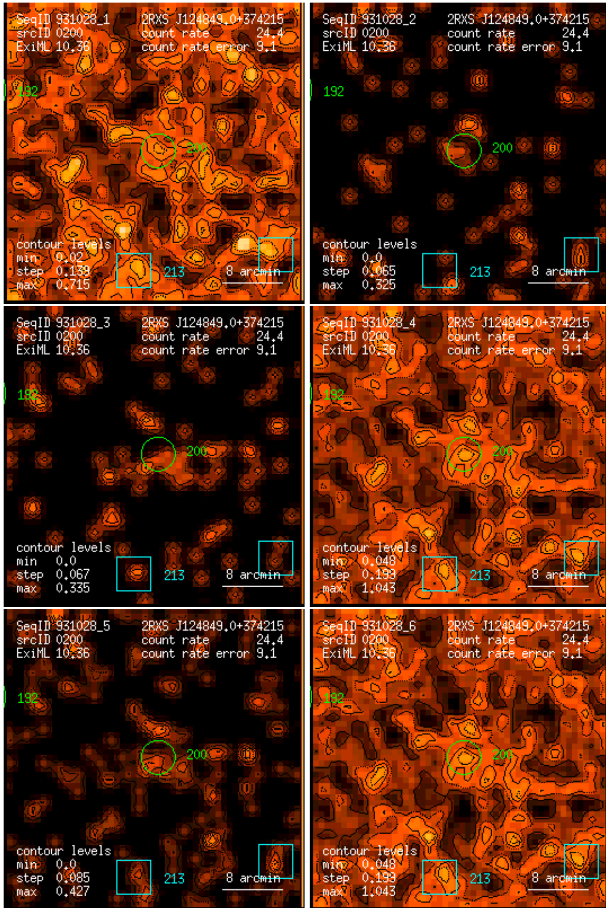
Figure 200: RASS 931028: detection 0200: band rate images, Gaussian filter: (1) PSPC channels 11 – 41, (2) 52 – 90, (3) 91 – 201, (4) 11 – 235, (5) 52 – 201, (6) 11 – 201. Broad band rates in counts/ks. Band rate contour levels in counts/ks/arcmin 2 .
