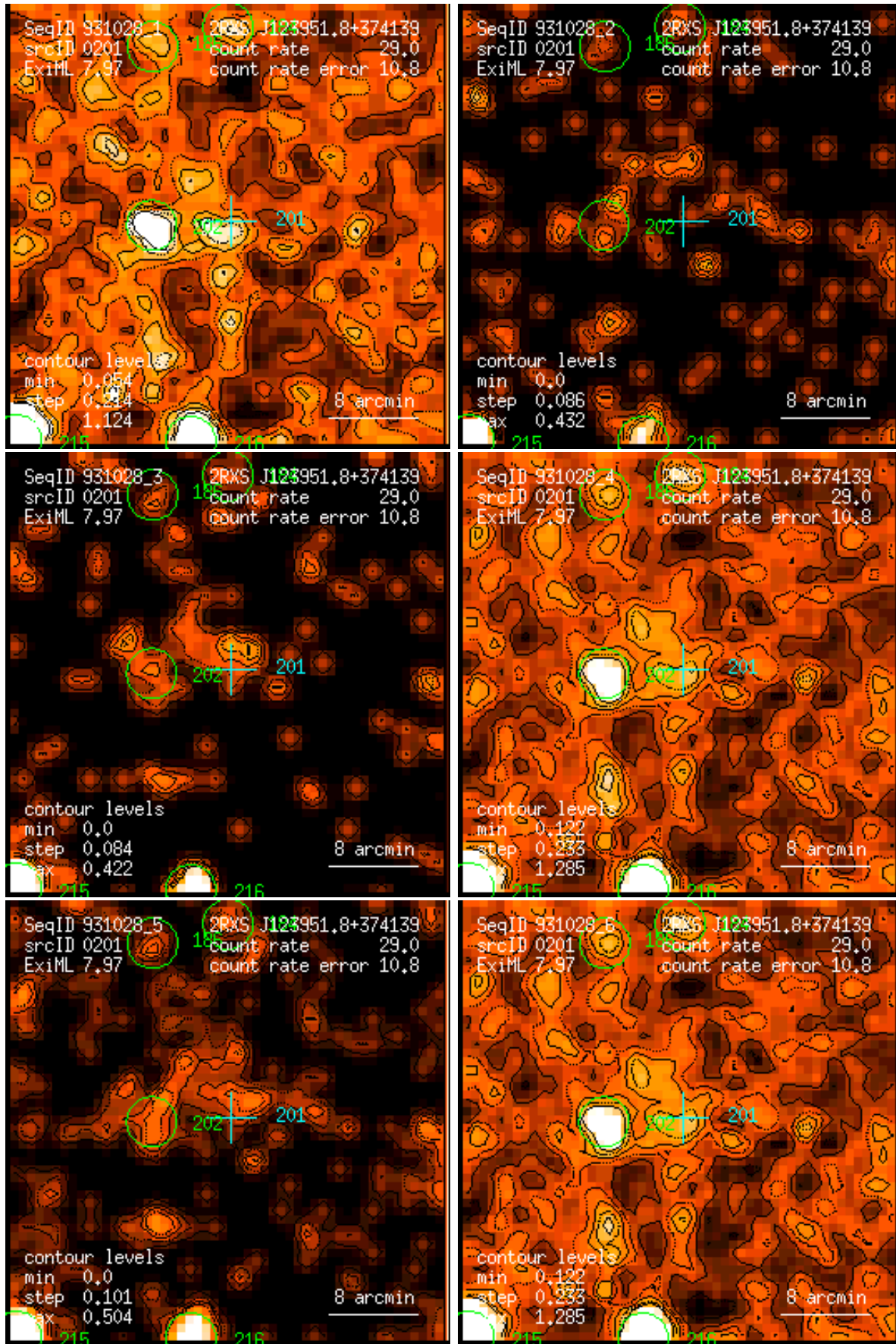
Figure 201: RASS 931028: detection 0201: band rate images, Gaussian filter: (1) PSPC channels 11 – 41, (2) 52 – 90, (3) 91 – 201, (4) 11 – 235, (5) 52 – 201, (6) 11 – 201. Broad band rates in counts/ks. Band rate contour levels in counts/ks/arcmin 2 .
