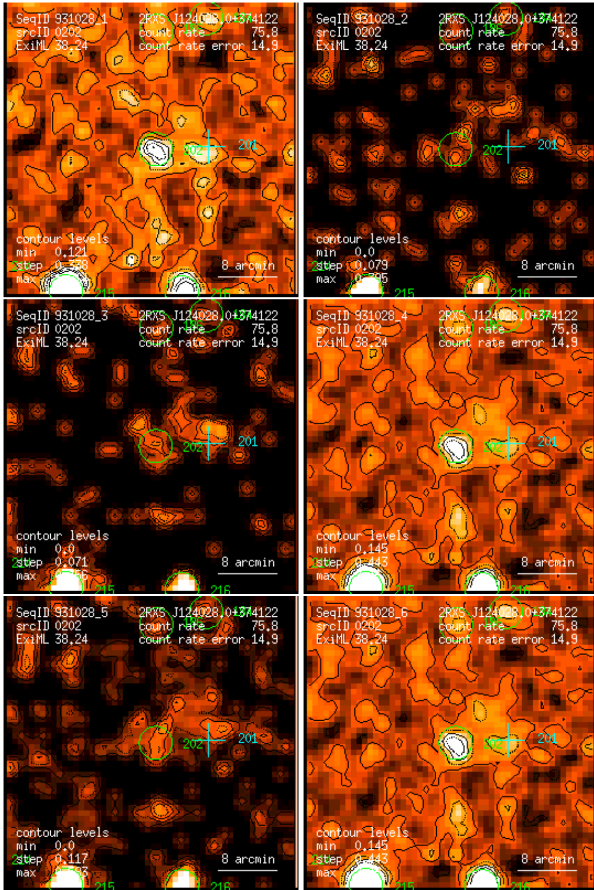
Figure 202: RASS 931028: detection 0202: band rate images, Gaussian filter: (1) PSPC channels 11 – 41, (2) 52 – 90, (3) 91 – 201, (4) 11 – 235, (5) 52 – 201, (6) 11 – 201. Broad band rates in counts/ks. Band rate contour levels in counts/ks/arcmin 2 .
