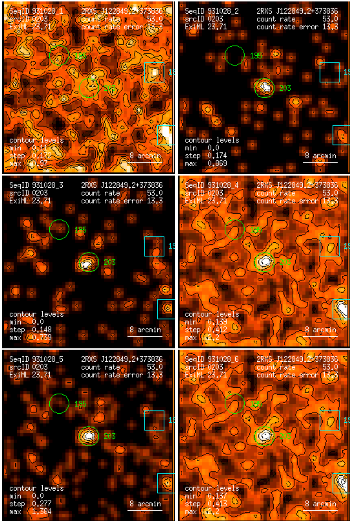
Figure 203: RASS 931028: detection 0203: band rate images, Gaussian filter: (1) PSPC channels 11 – 41, (2) 52 – 90, (3) 91 – 201, (4) 11 – 235, (5) 52 – 201, (6) 11 – 201. Broad band rates in counts/ks. Band rate contour levels in counts/ks/arcmin 2 .
