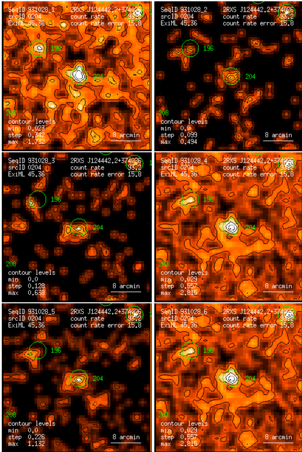
Figure 204: RASS 931028: detection 0204: band rate images, Gaussian filter: (1) PSPC channels 11 – 41, (2) 52 – 90, (3) 91 – 201, (4) 11 – 235, (5) 52 – 201, (6) 11 – 201. Broad band rates in counts/ks. Band rate contour levels in counts/ks/arcmin 2 .
