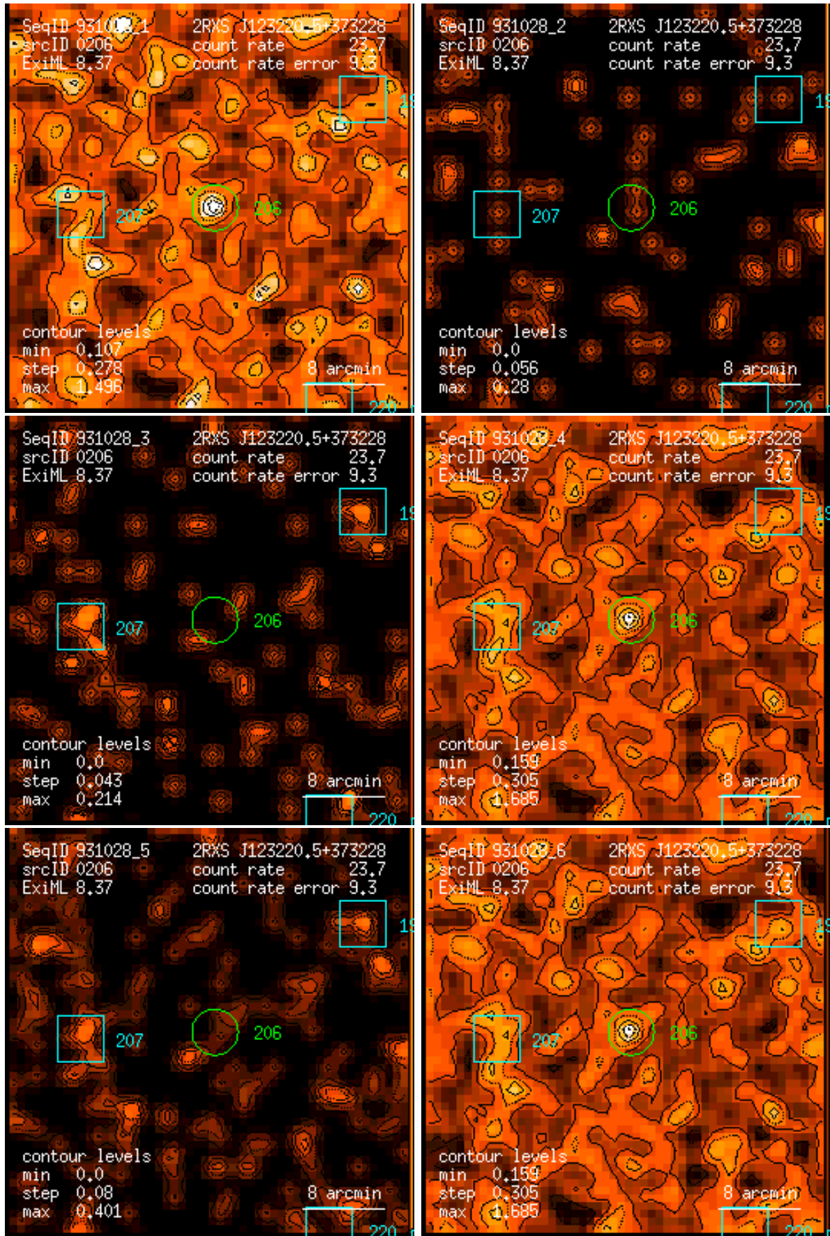
Figure 206: RASS 931028: detection 0206: band rate images, Gaussian filter: (1) PSPC channels 11 – 41, (2) 52 – 90, (3) 91 – 201, (4) 11 – 235, (5) 52 – 201, (6) 11 – 201. Broad band rates in counts/ks. Band rate contour levels in counts/ks/arcmin 2 .
