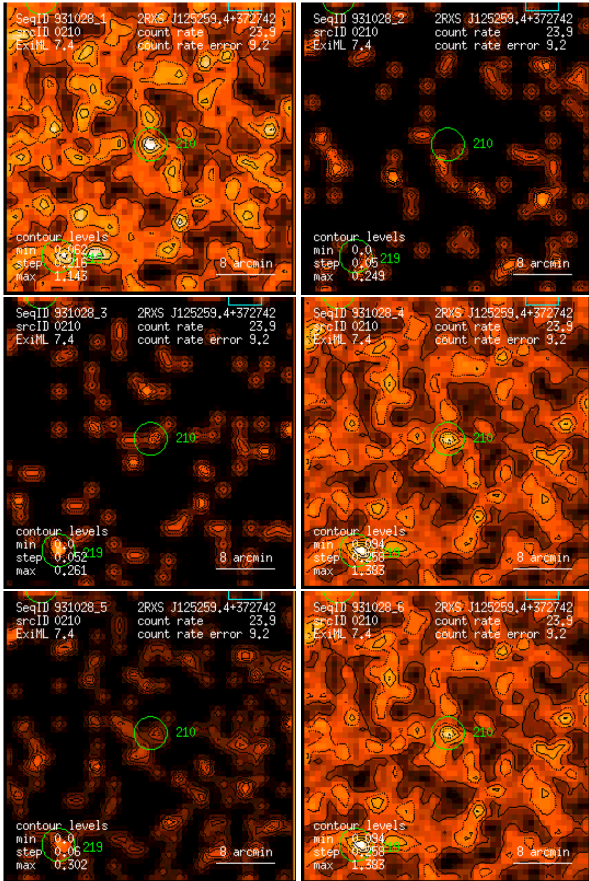
Figure 210: RASS 931028: detection 0210: band rate images, Gaussian filter: (1) PSPC channels 11 – 41, (2) 52 – 90, (3) 91 – 201, (4) 11 – 235, (5) 52 – 201, (6) 11 – 201. Broad band rates in counts/ks. Band rate contour levels in counts/ks/arcmin 2 .
