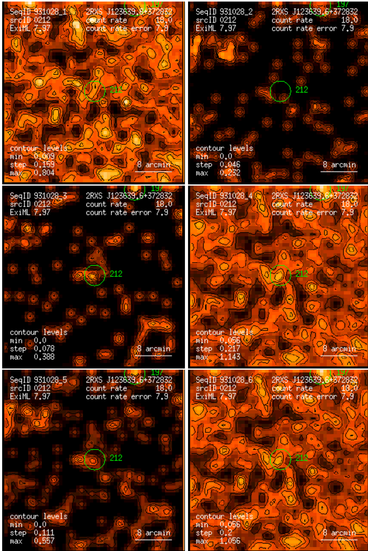
Figure 212: RASS 931028: detection 0212: band rate images, Gaussian filter: (1) PSPC channels 11 – 41, (2) 52 – 90, (3) 91 – 201, (4) 11 – 235, (5) 52 – 201, (6) 11 – 201. Broad band rates in counts/ks. Band rate contour levels in counts/ks/arcmin 2 .
