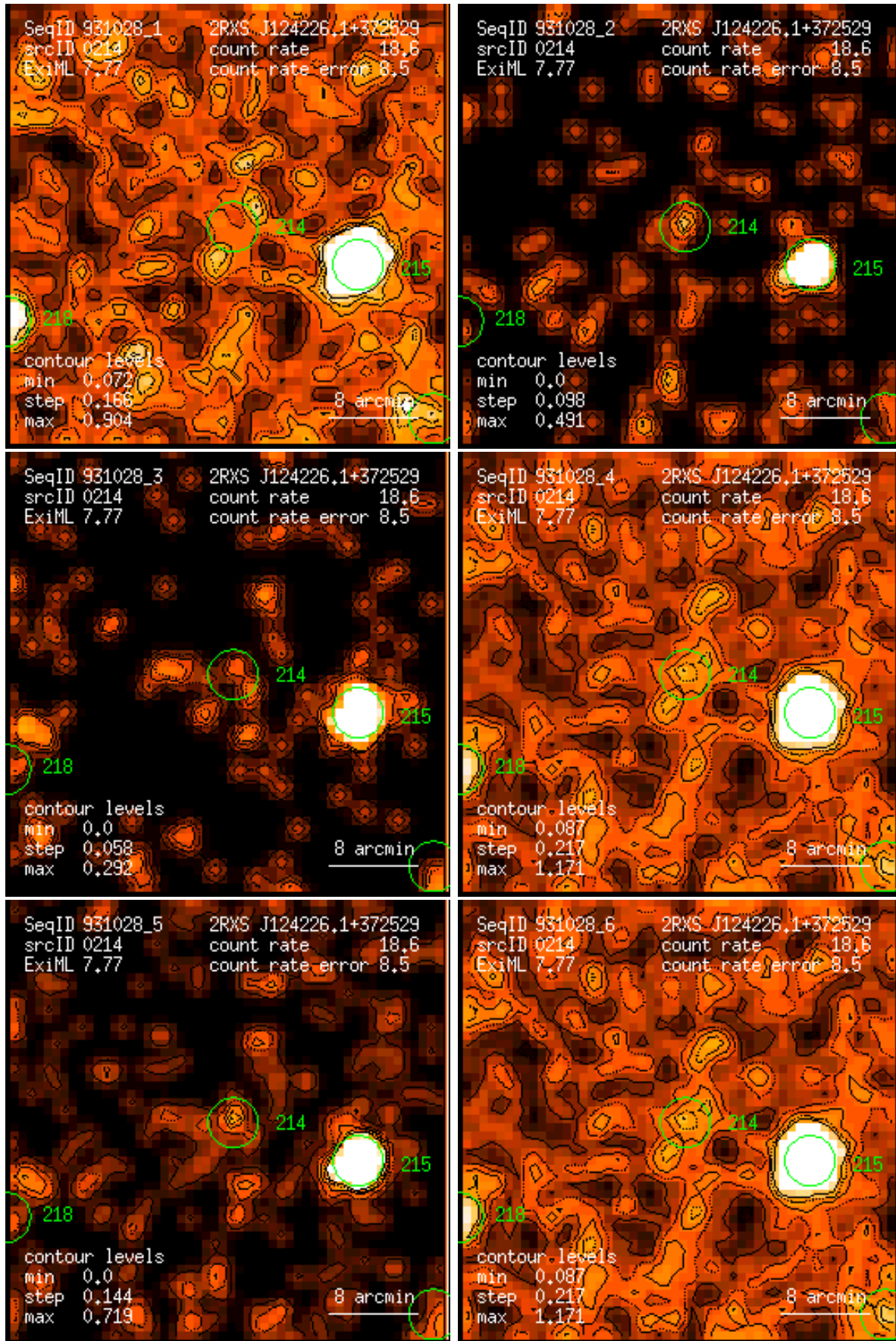
Figure 214: RASS 931028: detection 0214: band rate images, Gaussian filter: (1) PSPC channels 11 – 41, (2) 52 – 90, (3) 91 – 201, (4) 11 – 235, (5) 52 – 201, (6) 11 – 201. Broad band rates in counts/ks. Band rate contour levels in counts/ks/arcmin 2 .
