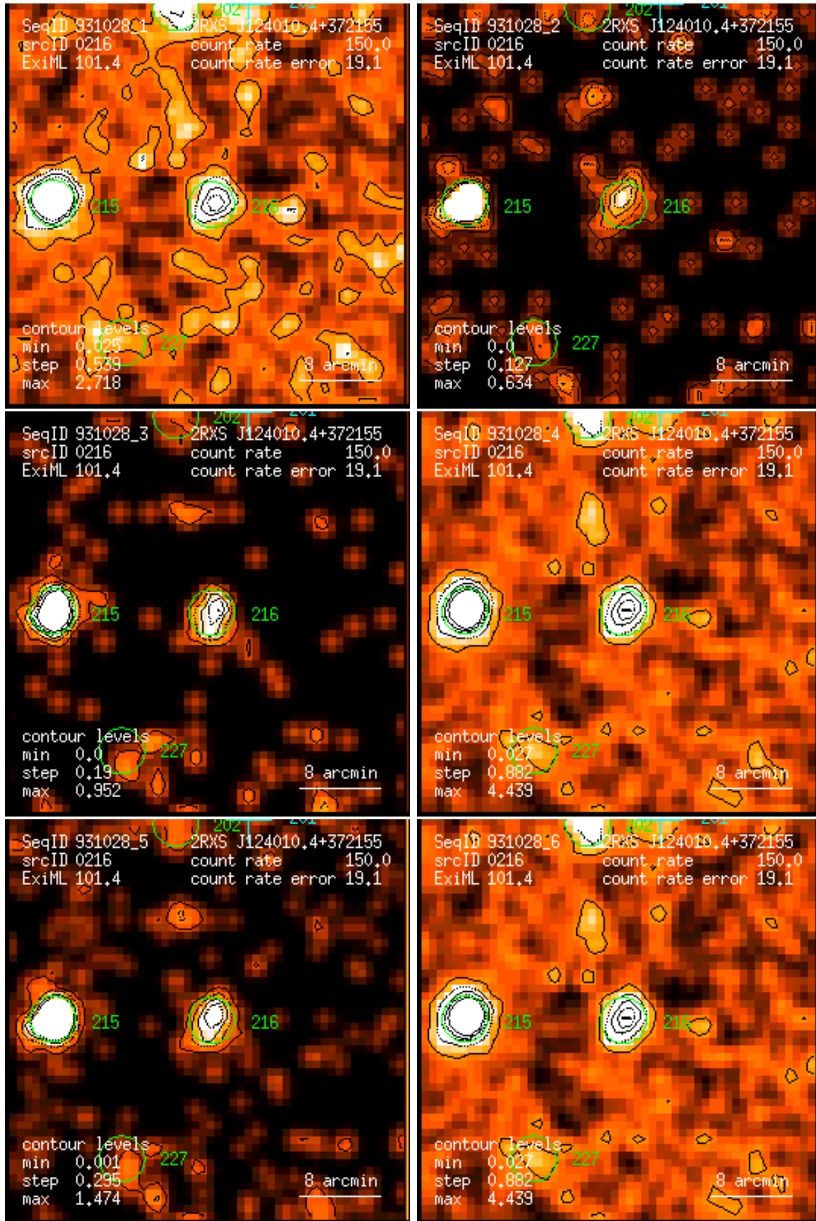
Figure 216: RASS 931028: detection 0216: band rate images, Gaussian filter: (1) PSPC channels 11 – 41, (2) 52 – 90, (3) 91 – 201, (4) 11 – 235, (5) 52 – 201, (6) 11 – 201. Broad band rates in counts/ks. Band rate contour levels in counts/ks/arcmin 2 .
