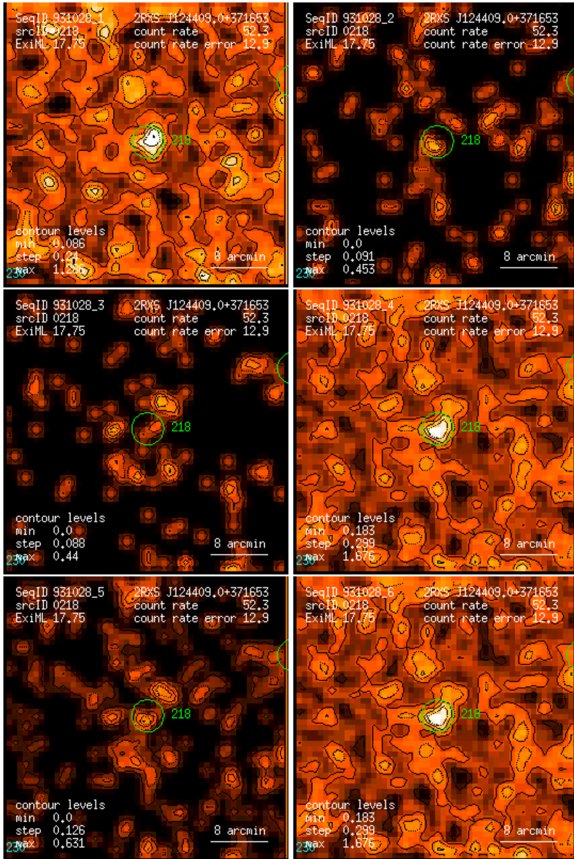
Figure 218: RASS 931028: detection 0218: band rate images, Gaussian filter: (1) PSPC channels 11 – 41, (2) 52 – 90, (3) 91 – 201, (4) 11 – 235, (5) 52 – 201, (6) 11 – 201. Broad band rates in counts/ks. Band rate contour levels in counts/ks/arcmin 2 .
