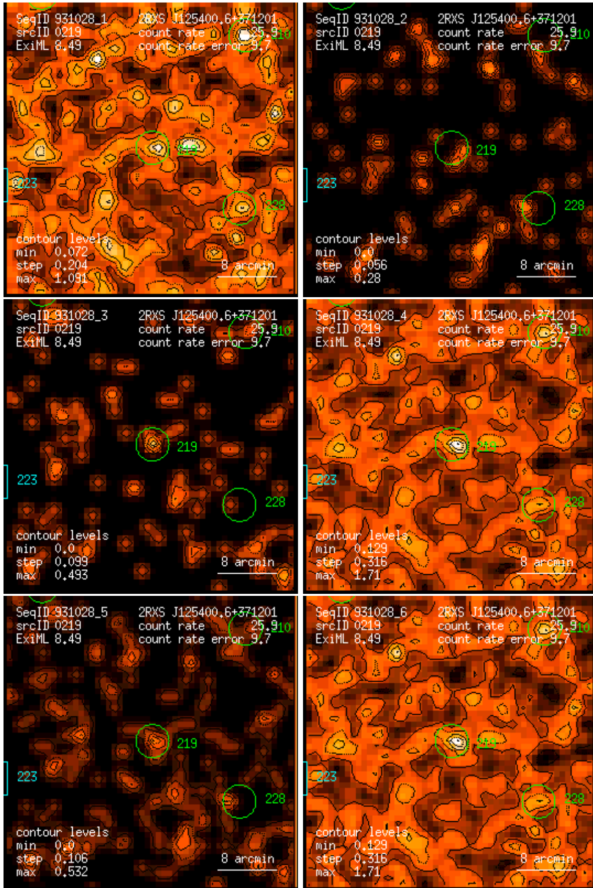
Figure 219: RASS 931028: detection 0219: band rate images, Gaussian filter: (1) PSPC channels 11 – 41, (2) 52 – 90, (3) 91 – 201, (4) 11 – 235, (5) 52 – 201, (6) 11 – 201. Broad band rates in counts/ks. Band rate contour levels in counts/ks/arcmin 2 .
