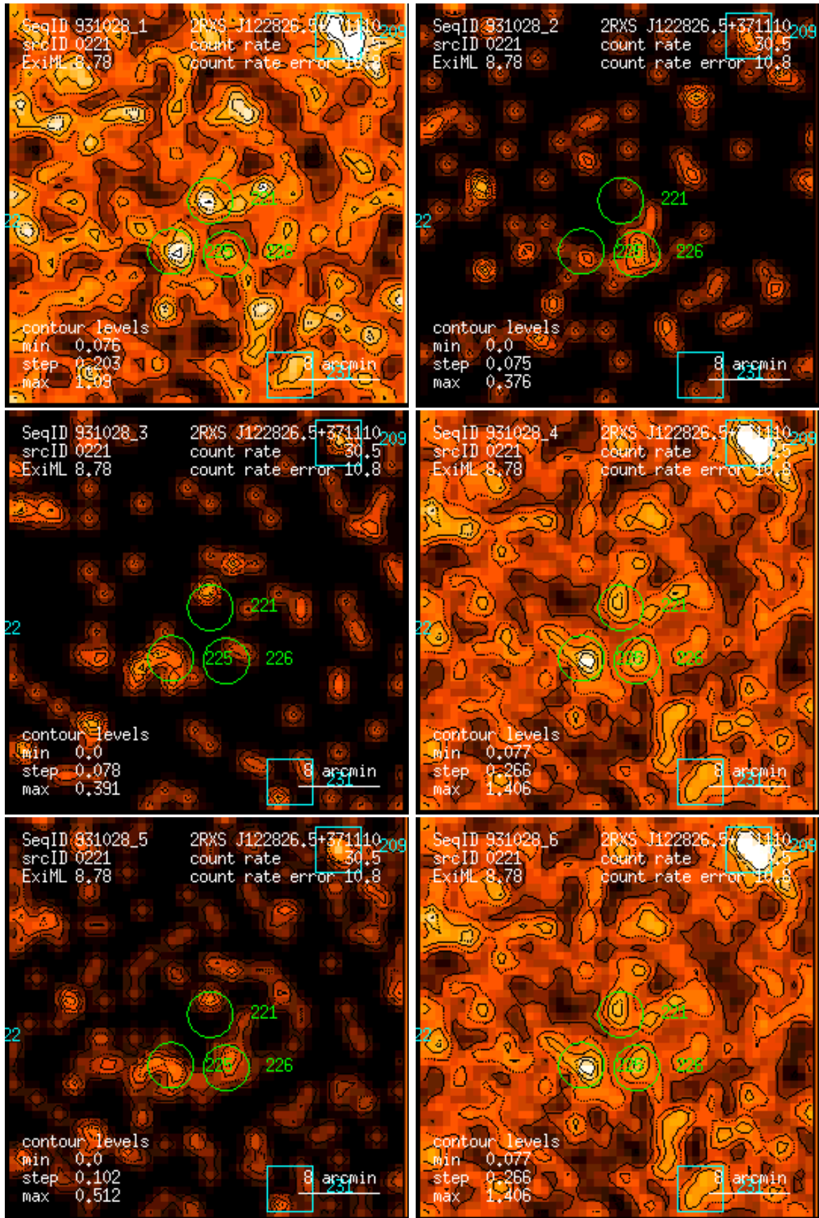
Figure 221: RASS 931028: detection 0221: band rate images, Gaussian filter: (1) PSPC channels 11 – 41, (2) 52 – 90, (3) 91 – 201, (4) 11 – 235, (5) 52 – 201, (6) 11 – 201. Broad band rates in counts/ks. Band rate contour levels in counts/ks/arcmin 2 .
