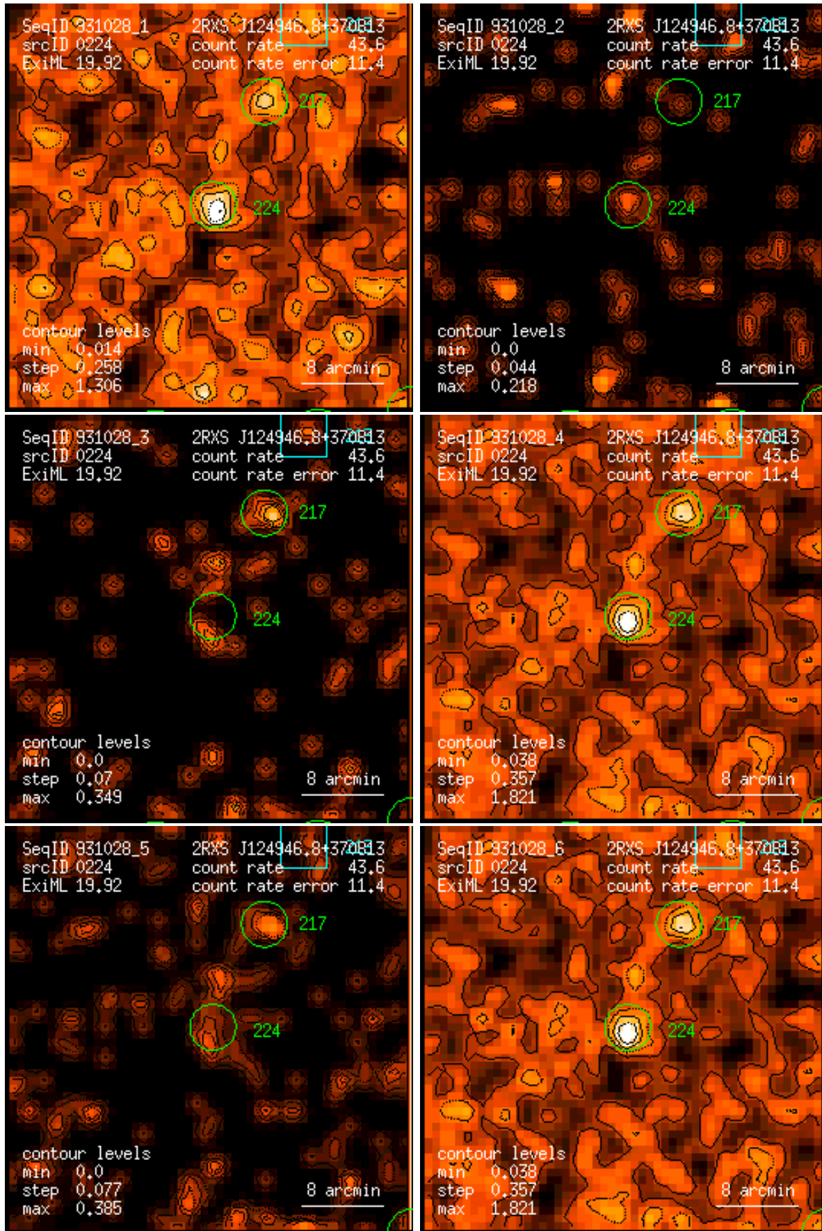
Figure 224: RASS 931028: detection 0224: band rate images, Gaussian filter: (1) PSPC channels 11 – 41, (2) 52 – 90, (3) 91 – 201, (4) 11 – 235, (5) 52 – 201, (6) 11 – 201. Broad band rates in counts/ks. Band rate contour levels in counts/ks/arcmin 2 .
