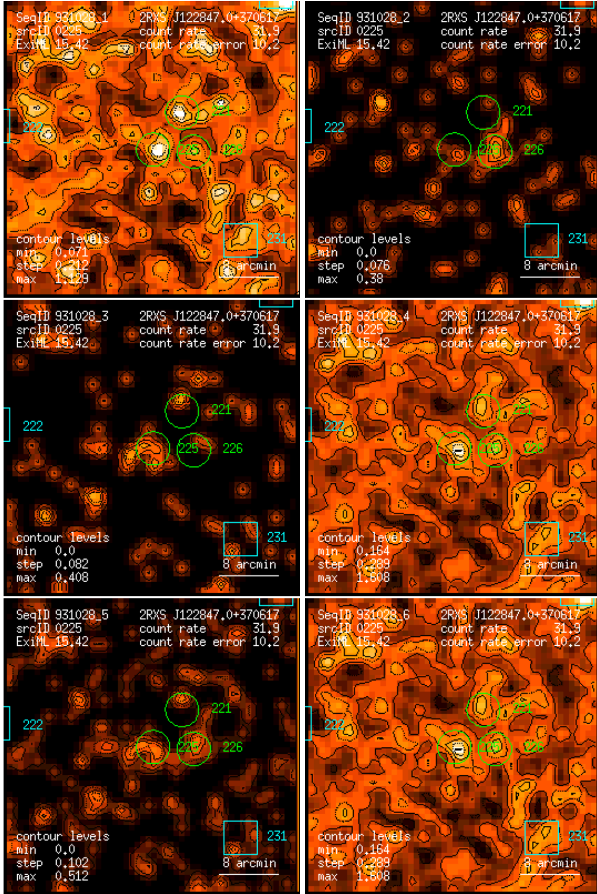
Figure 225: RASS 931028: detection 0225: band rate images, Gaussian filter: (1) PSPC channels 11 – 41, (2) 52 – 90, (3) 91 – 201, (4) 11 – 235, (5) 52 – 201, (6) 11 – 201. Broad band rates in counts/ks. Band rate contour levels in counts/ks/arcmin 2 .
