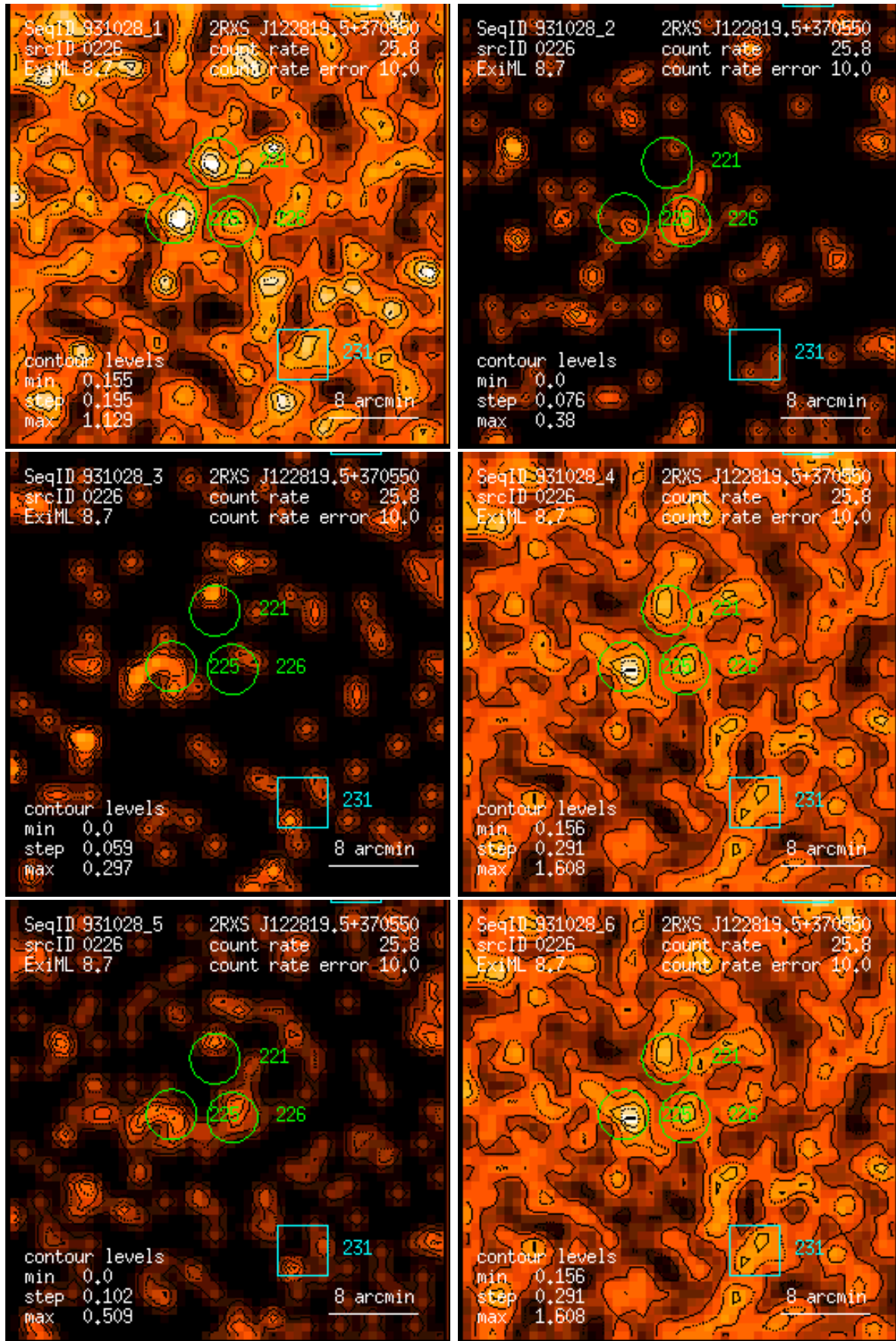
Figure 226: RASS 931028: detection 0226: band rate images, Gaussian filter: (1) PSPC channels 11 – 41, (2) 52 – 90, (3) 91 – 201, (4) 11 – 235, (5) 52 – 201, (6) 11 – 201. Broad band rates in counts/ks. Band rate contour levels in counts/ks/arcmin 2 .
