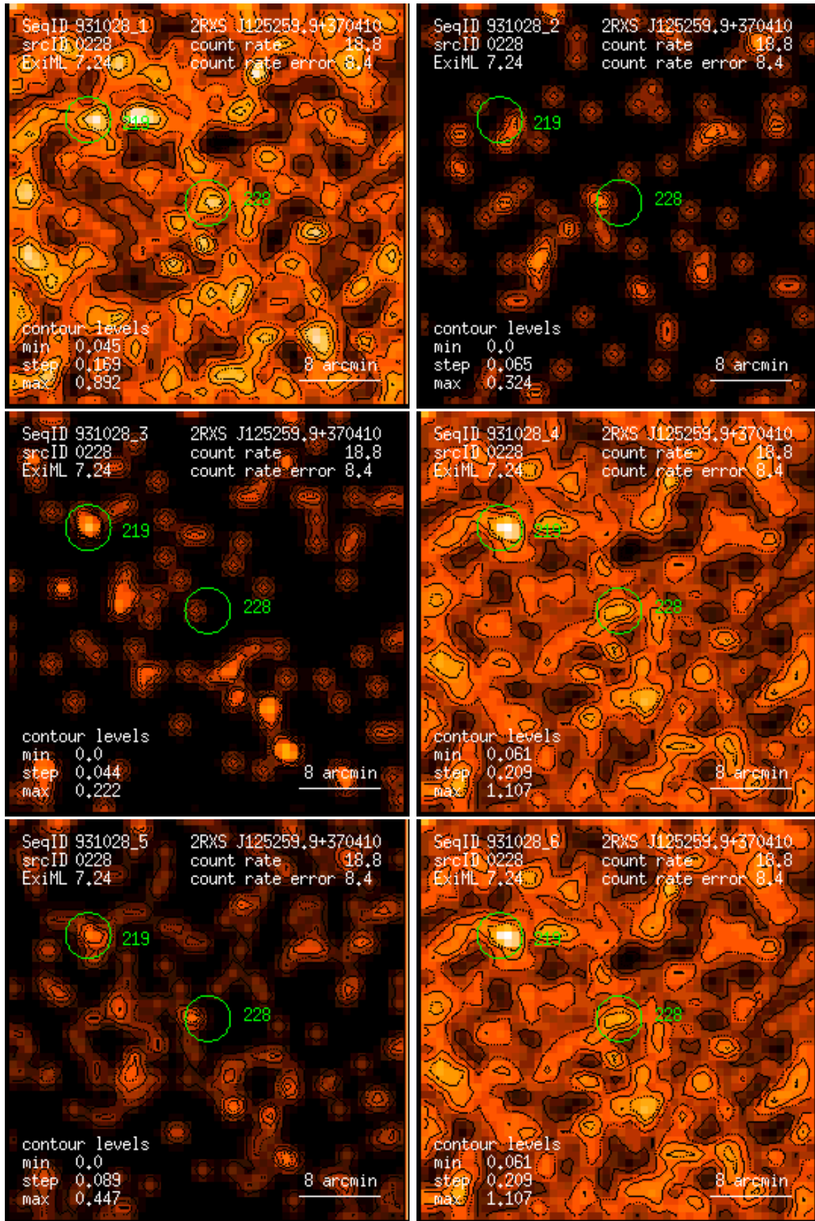
Figure 228: RASS 931028: detection 0228: band rate images, Gaussian filter: (1) PSPC channels 11 – 41, (2) 52 – 90, (3) 91 – 201, (4) 11 – 235, (5) 52 – 201, (6) 11 – 201. Broad band rates in counts/ks. Band rate contour levels in counts/ks/arcmin 2 .
