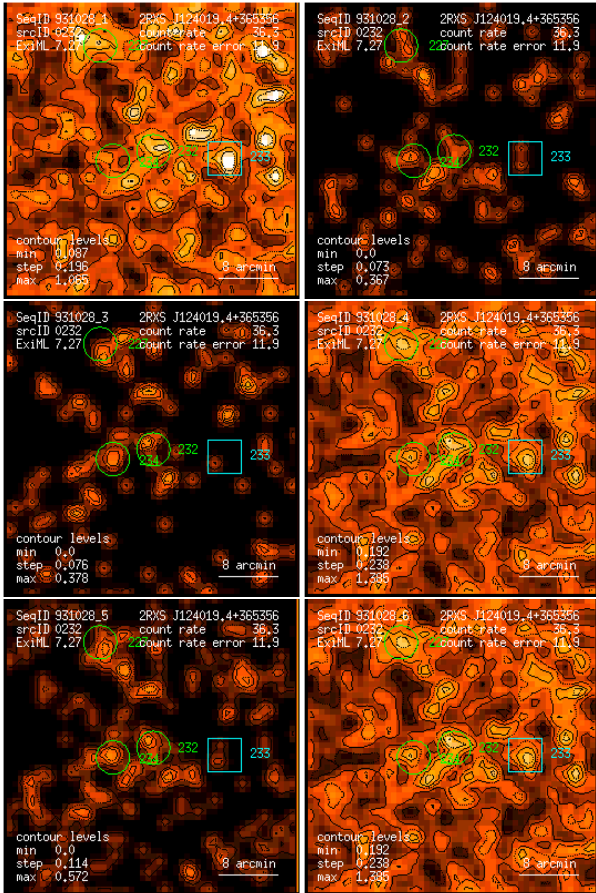
Figure 232: RASS 931028: detection 0232: band rate images, Gaussian filter: (1) PSPC channels 11 – 41, (2) 52 – 90, (3) 91 – 201, (4) 11 – 235, (5) 52 – 201, (6) 11 – 201. Broad band rates in counts/ks. Band rate contour levels in counts/ks/arcmin 2 .
