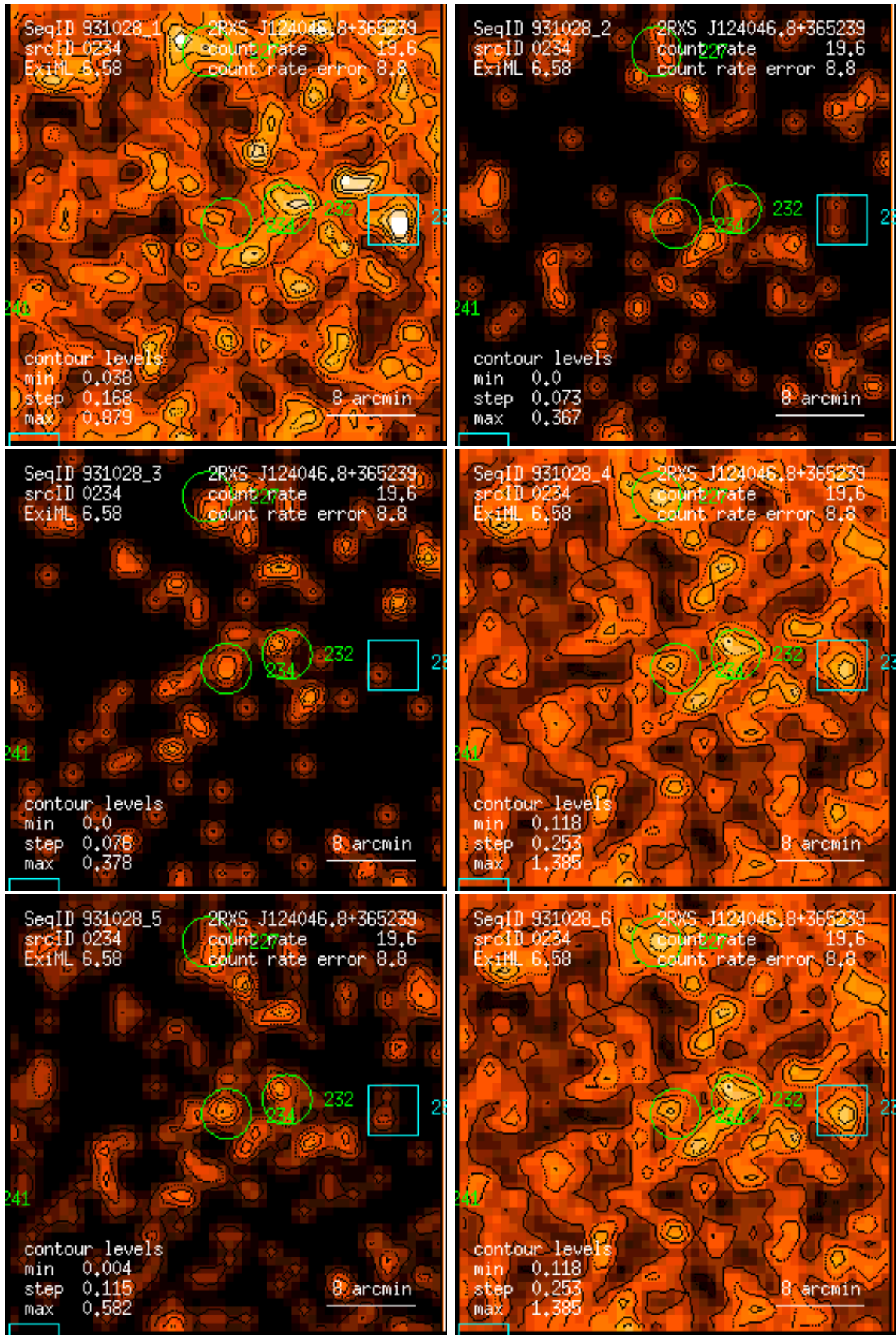
Figure 234: RASS 931028: detection 0234: band rate images, Gaussian filter: (1) PSPC channels 11 – 41, (2) 52 – 90, (3) 91 – 201, (4) 11 – 235, (5) 52 – 201, (6) 11 – 201. Broad band rates in counts/ks. Band rate contour levels in counts/ks/arcmin 2 .
