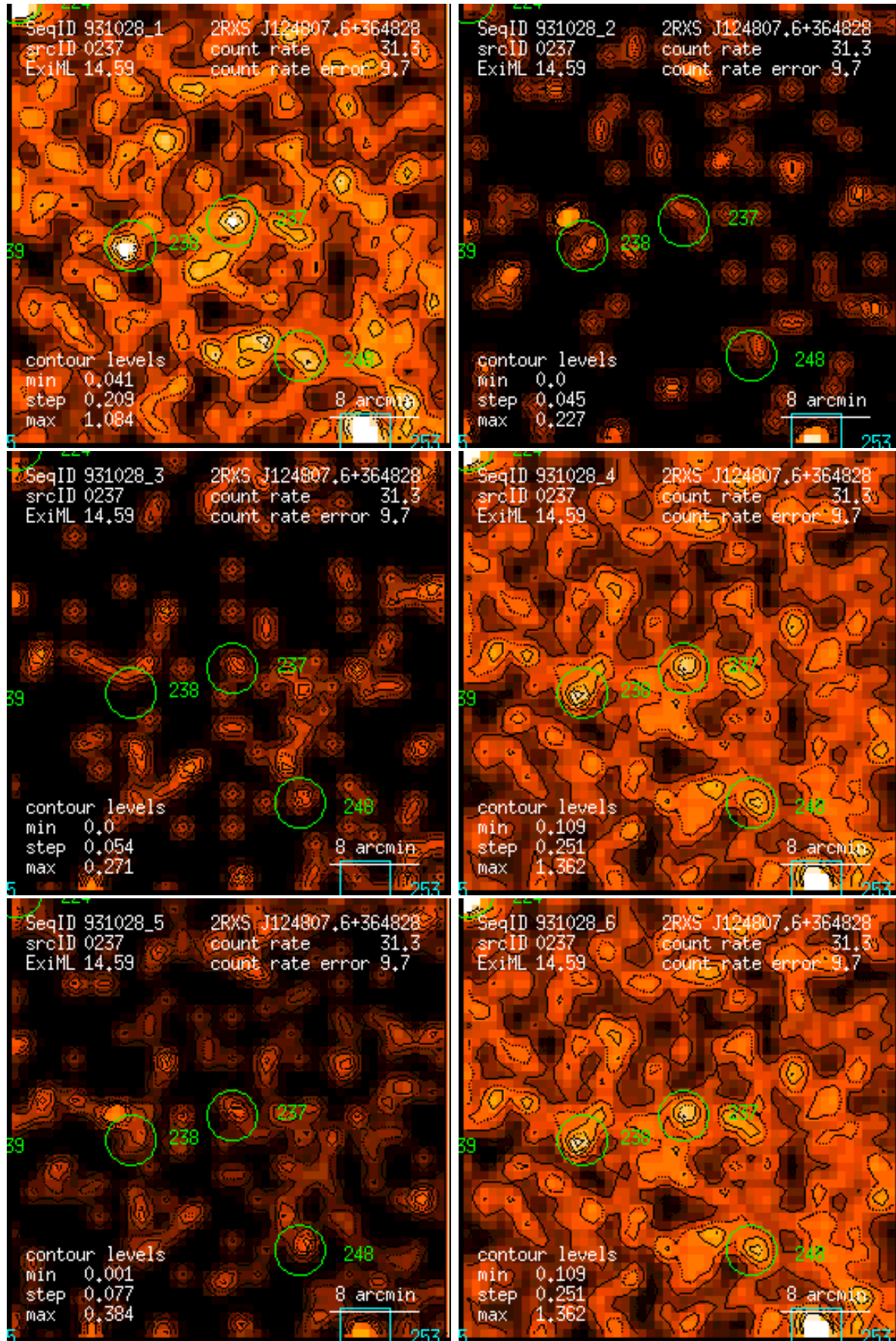
Figure 237: RASS 931028: detection 0237: band rate images, Gaussian filter: (1) PSPC channels 11 – 41, (2) 52 – 90, (3) 91 – 201, (4) 11 – 235, (5) 52 – 201, (6) 11 – 201. Broad band rates in counts/ks. Band rate contour levels in counts/ks/arcmin 2 .
