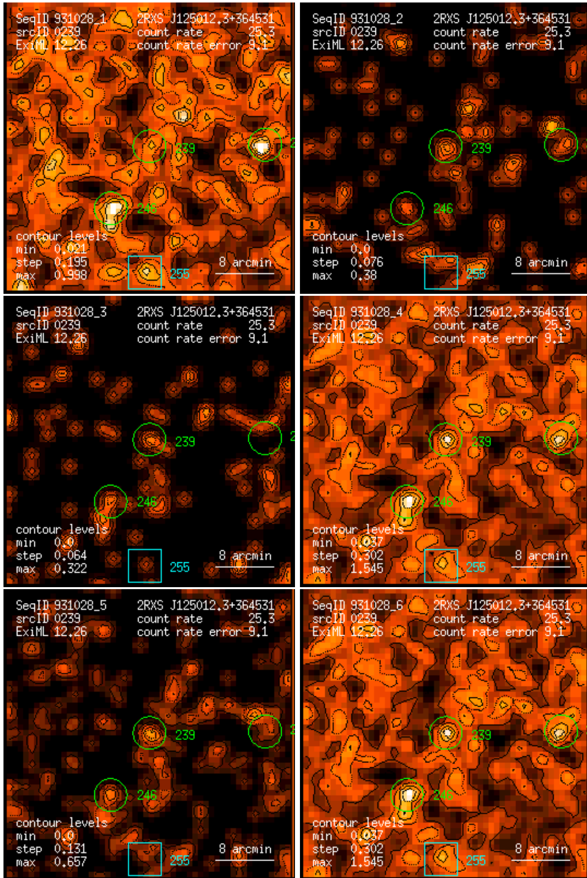
Figure 239: RASS 931028: detection 0239: band rate images, Gaussian filter: (1) PSPC channels 11 – 41, (2) 52 – 90, (3) 91 – 201, (4) 11 – 235, (5) 52 – 201, (6) 11 – 201. Broad band rates in counts/ks. Band rate contour levels in counts/ks/arcmin 2 .
