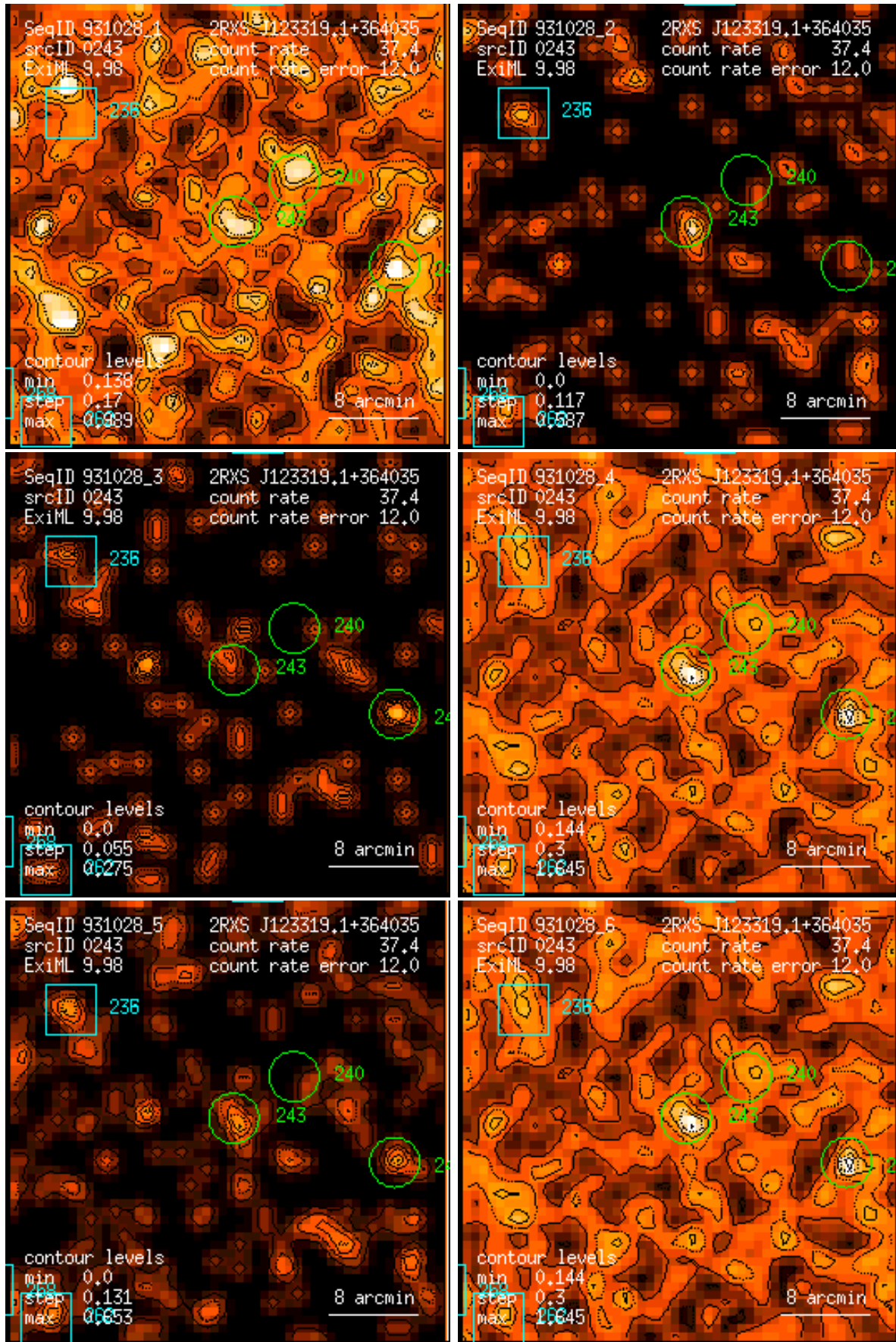
Figure 243: RASS 931028: detection 0243: band rate images, Gaussian filter: (1) PSPC channels 11 – 41, (2) 52 – 90, (3) 91 – 201, (4) 11 – 235, (5) 52 – 201, (6) 11 – 201. Broad band rates in counts/ks. Band rate contour levels in counts/ks/arcmin 2 .
