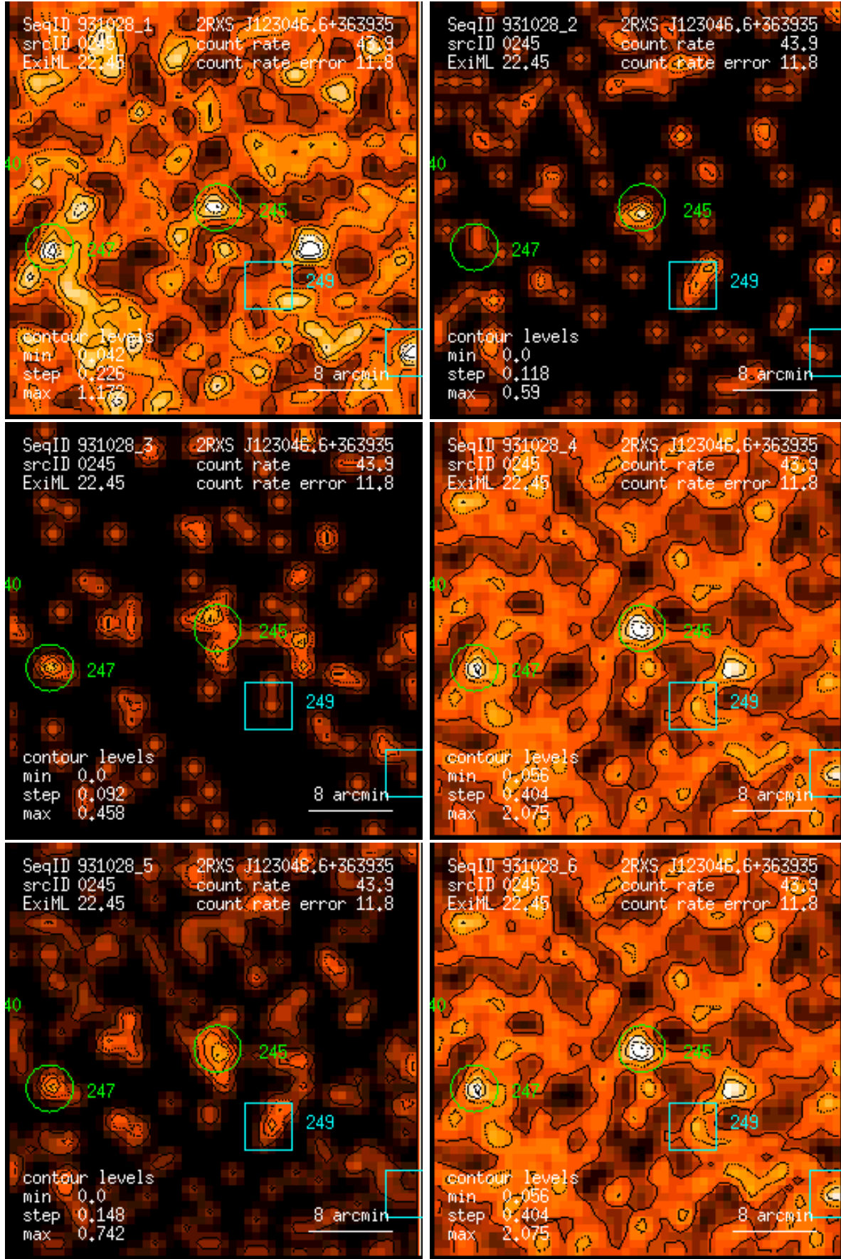
Figure 245: RASS 931028: detection 0245: band rate images, Gaussian filter: (1) PSPC channels 11 – 41, (2) 52 – 90, (3) 91 – 201, (4) 11 – 235, (5) 52 – 201, (6) 11 – 201. Broad band rates in counts/ks. Band rate contour levels in counts/ks/arcmin 2 .
