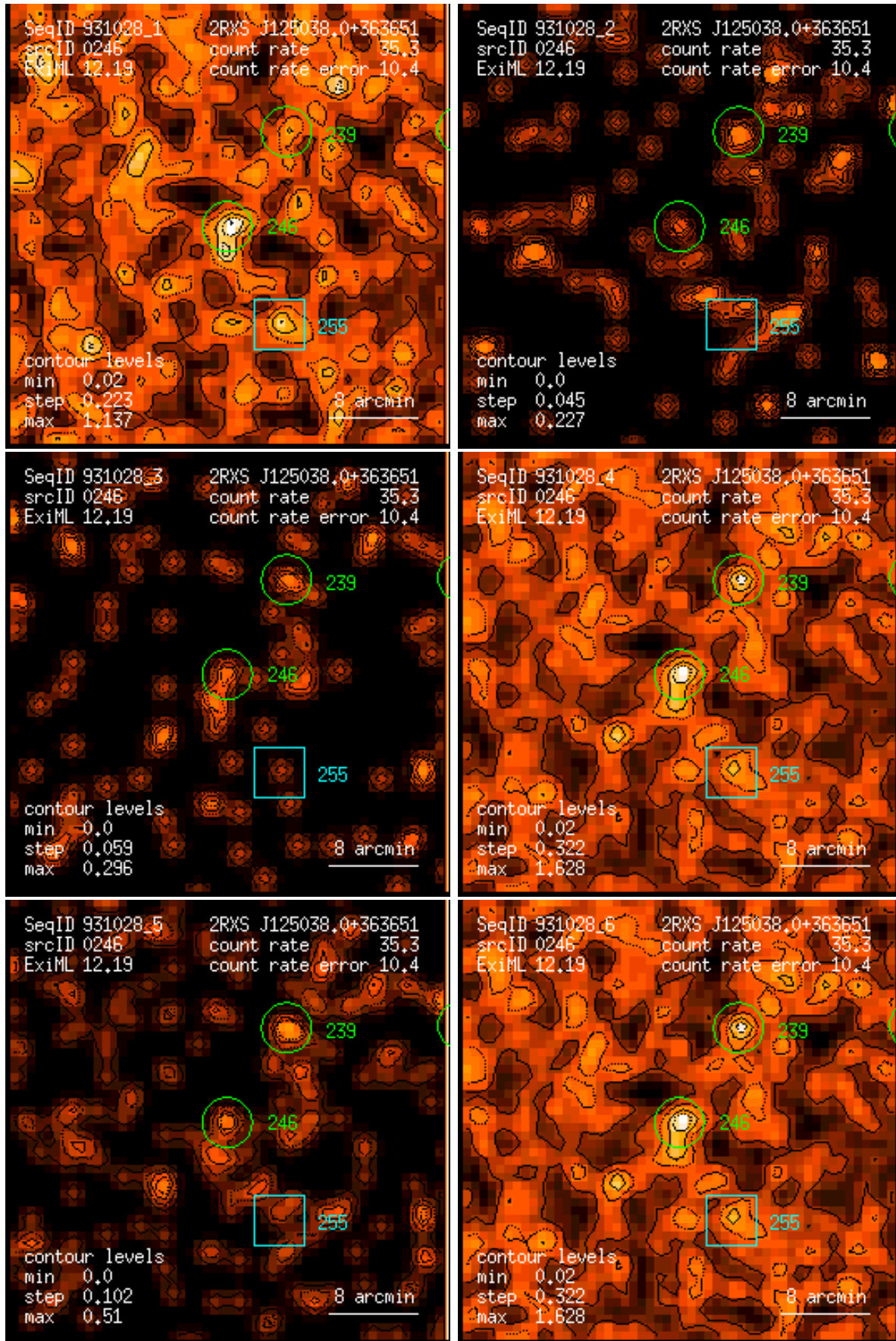
Figure 246: RASS 931028: detection 0246: band rate images, Gaussian filter: (1) PSPC channels 11 – 41, (2) 52 – 90, (3) 91 – 201, (4) 11 – 235, (5) 52 – 201, (6) 11 – 201. Broad band rates in counts/ks. Band rate contour levels in counts/ks/arcmin 2 .
