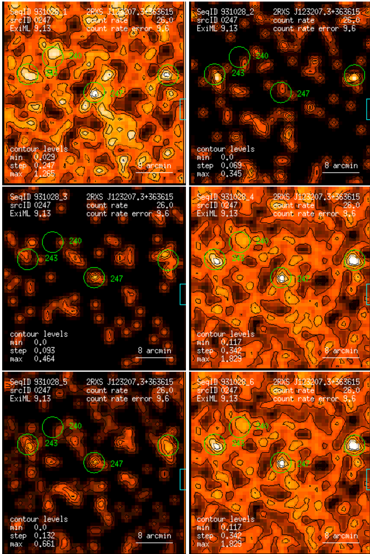
Figure 247: RASS 931028: detection 0247: band rate images, Gaussian filter: (1) PSPC channels 11 – 41, (2) 52 – 90, (3) 91 – 201, (4) 11 – 235, (5) 52 – 201, (6) 11 – 201. Broad band rates in counts/ks. Band rate contour levels in counts/ks/arcmin 2 .
