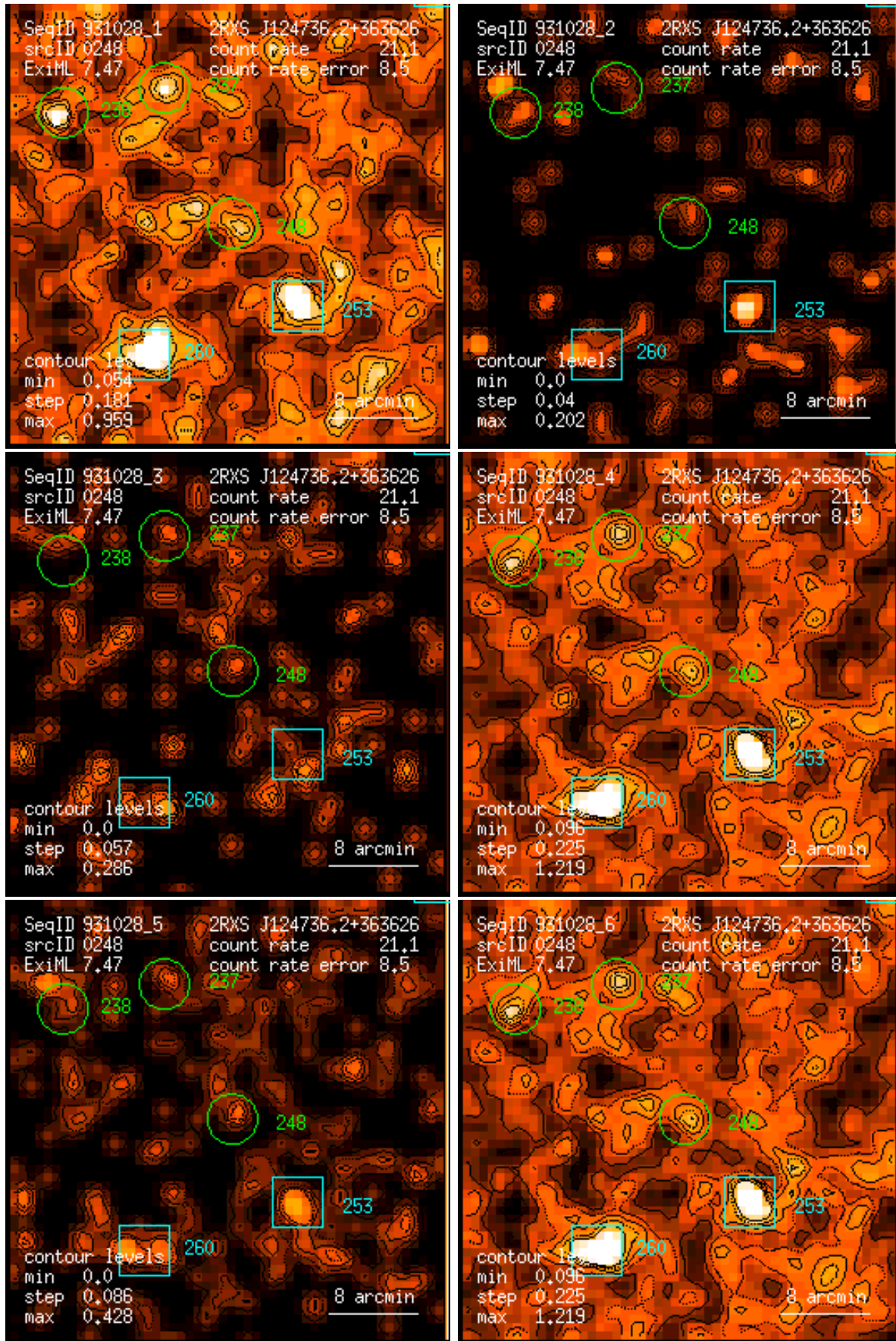
Figure 248: RASS 931028: detection 0248: band rate images, Gaussian filter: (1) PSPC channels 11 – 41, (2) 52 – 90, (3) 91 – 201, (4) 11 – 235, (5) 52 – 201, (6) 11 – 201. Broad band rates in counts/ks. Band rate contour levels in counts/ks/arcmin 2 .
