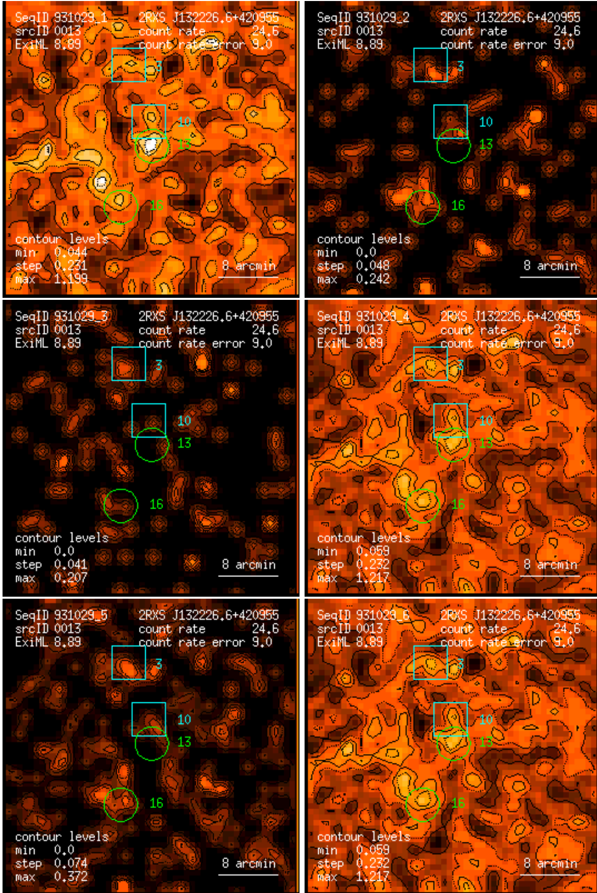
Figure 13: RASS 931029: detection 0013: band rate images, Gaussian filter: (1) PSPC channels 11 – 41, (2) 52 – 90, (3) 91 – 201, (4) 11 – 235, (5) 52 – 201, (6) 11 – 201. Broad band rates in counts/ks. Band rate contour levels in counts/ks/arcmin 2 .
