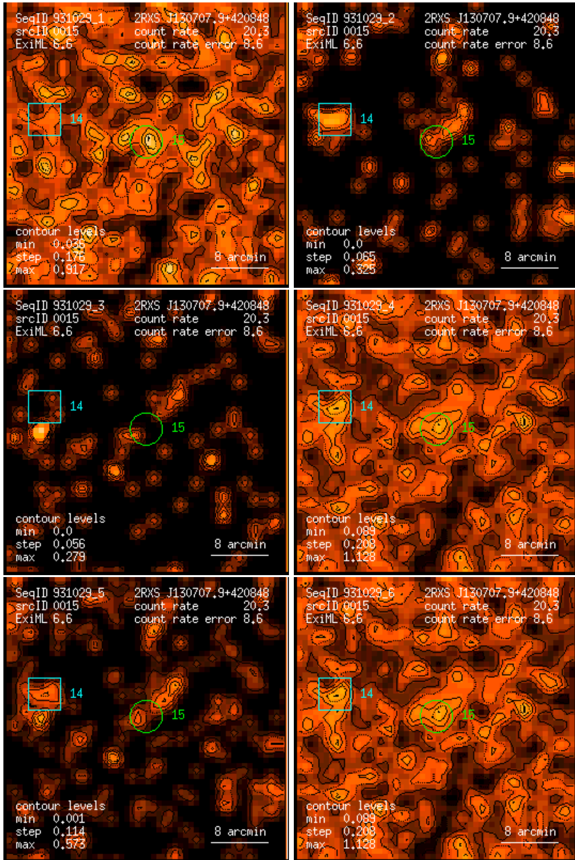
Figure 15: RASS 931029: detection 0015: band rate images, Gaussian filter: (1) PSPC channels 11 – 41, (2) 52 – 90, (3) 91 – 201, (4) 11 – 235, (5) 52 – 201, (6) 11 – 201. Broad band rates in counts/ks. Band rate contour levels in counts/ks/arcmin 2 .
