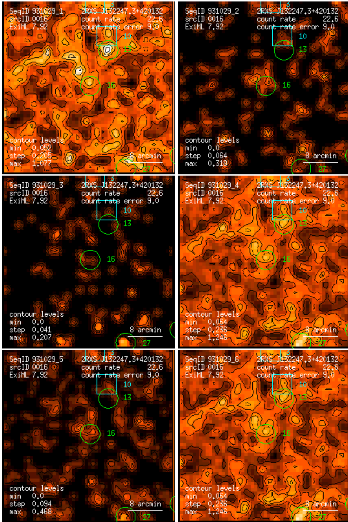
Figure 16: RASS 931029: detection 0016: band rate images, Gaussian filter: (1) PSPC channels 11 – 41, (2) 52 – 90, (3) 91 – 201, (4) 11 – 235, (5) 52 – 201, (6) 11 – 201. Broad band rates in counts/ks. Band rate contour levels in counts/ks/arcmin 2 .
