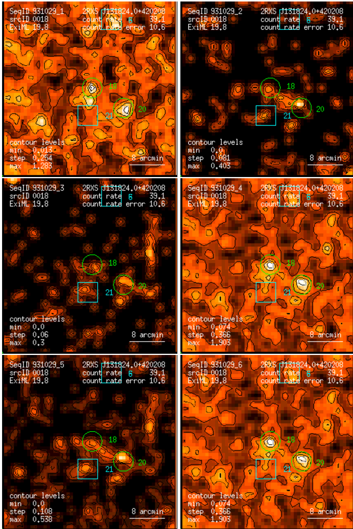
Figure 18: RASS 931029: detection 0018: band rate images, Gaussian filter: (1) PSPC channels 11 – 41, (2) 52 – 90, (3) 91 – 201, (4) 11 – 235, (5) 52 – 201, (6) 11 – 201. Broad band rates in counts/ks. Band rate contour levels in counts/ks/arcmin 2 .
