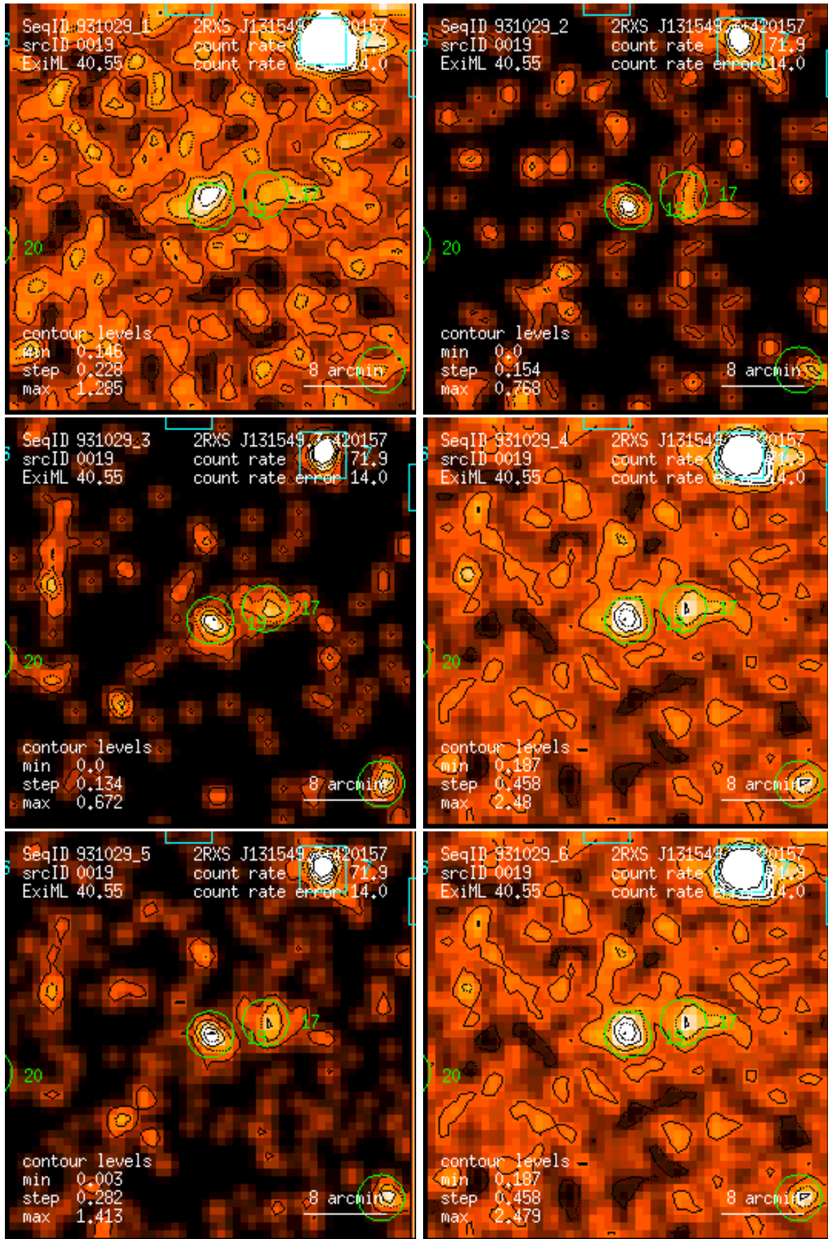
Figure 19: RASS 931029: detection 0019: band rate images, Gaussian filter: (1) PSPC channels 11 – 41, (2) 52 – 90, (3) 91 – 201, (4) 11 – 235, (5) 52 – 201, (6) 11 – 201. Broad band rates in counts/ks. Band rate contour levels in counts/ks/arcmin 2 .
