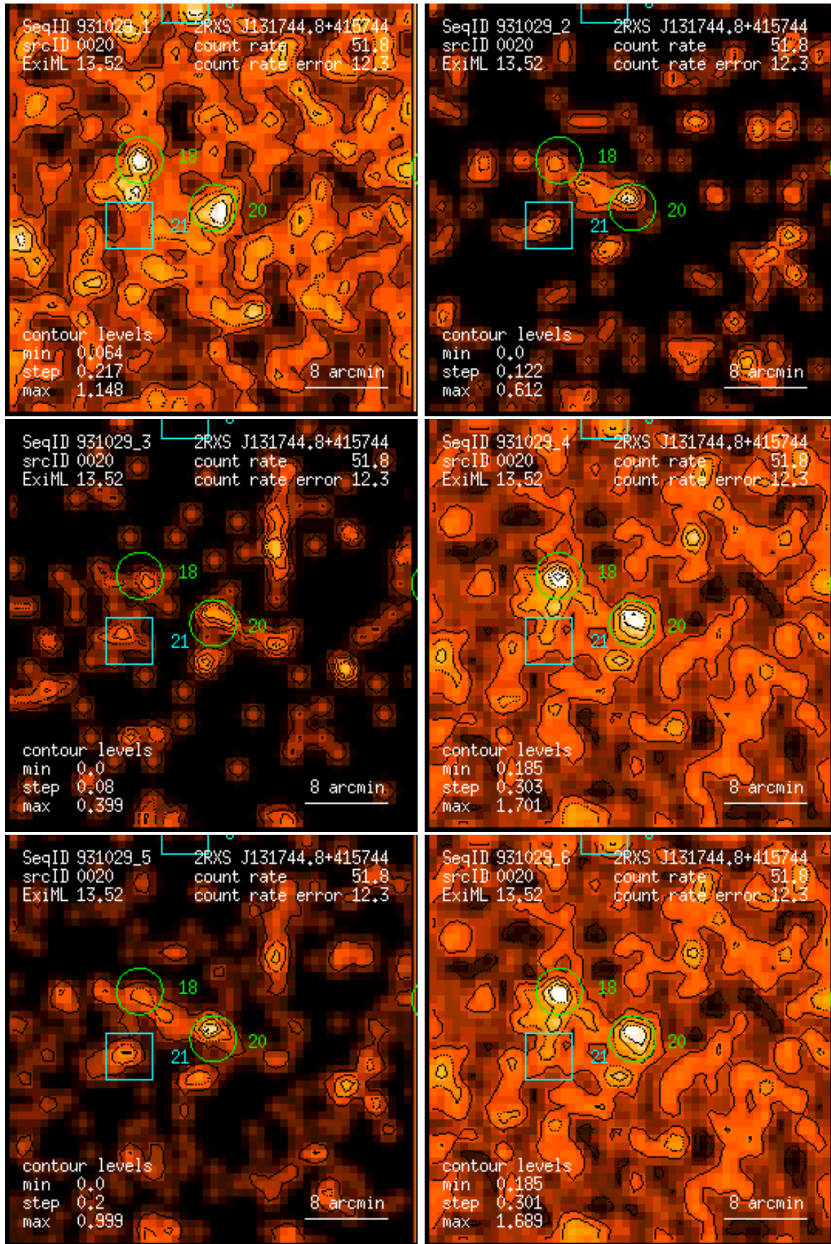
Figure 20: RASS 931029: detection 0020: band rate images, Gaussian filter: (1) PSPC channels 11 – 41, (2) 52 – 90, (3) 91 – 201, (4) 11 – 235, (5) 52 – 201, (6) 11 – 201. Broad band rates in counts/ks. Band rate contour levels in counts/ks/arcmin 2 .
