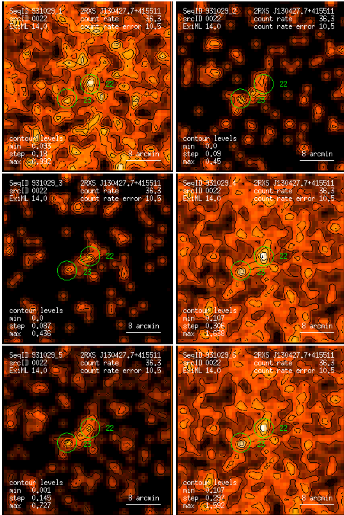
Figure 22: RASS 931029: detection 0022: band rate images, Gaussian filter: (1) PSPC channels 11 – 41, (2) 52 – 90, (3) 91 – 201, (4) 11 – 235, (5) 52 – 201, (6) 11 – 201. Broad band rates in counts/ks. Band rate contour levels in counts/ks/arcmin 2 .
