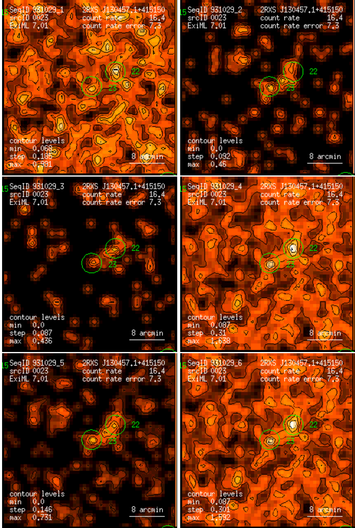
Figure 23: RASS 931029: detection 0023: band rate images, Gaussian filter: (1) PSPC channels 11 – 41, (2) 52 – 90, (3) 91 – 201, (4) 11 – 235, (5) 52 – 201, (6) 11 – 201. Broad band rates in counts/ks. Band rate contour levels in counts/ks/arcmin 2 .
