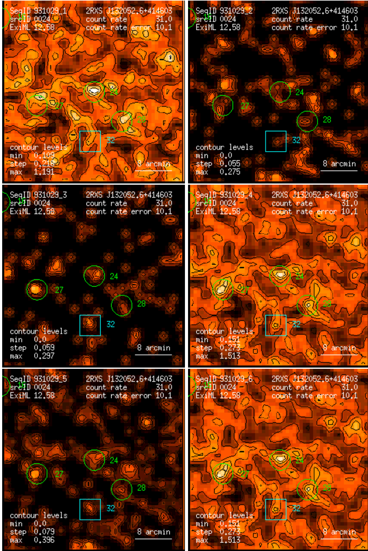
Figure 24: RASS 931029: detection 0024: band rate images, Gaussian filter: (1) PSPC channels 11 – 41, (2) 52 – 90, (3) 91 – 201, (4) 11 – 235, (5) 52 – 201, (6) 11 – 201. Broad band rates in counts/ks. Band rate contour levels in counts/ks/arcmin 2 .
