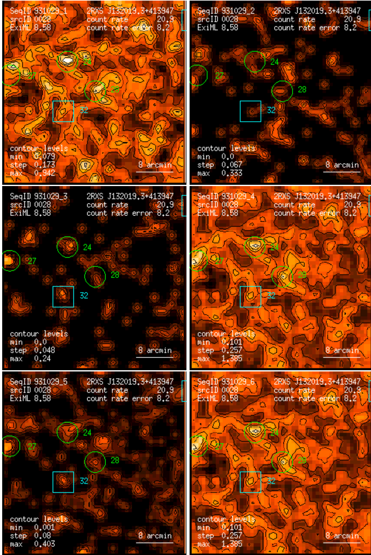
Figure 28: RASS 931029: detection 0028: band rate images, Gaussian filter: (1) PSPC channels 11 – 41, (2) 52 – 90, (3) 91 – 201, (4) 11 – 235, (5) 52 – 201, (6) 11 – 201. Broad band rates in counts/ks. Band rate contour levels in counts/ks/arcmin 2 .
