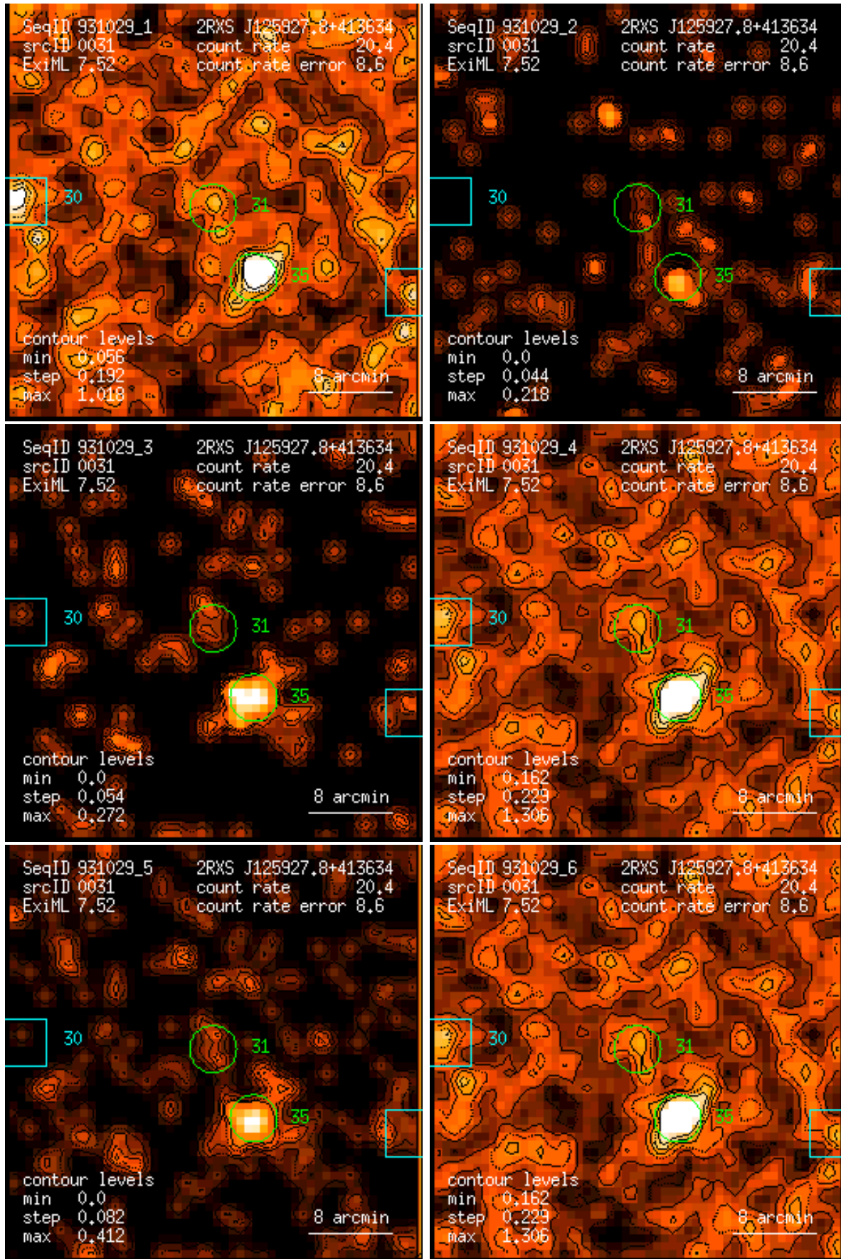
Figure 31: RASS 931029: detection 0031: band rate images, Gaussian filter: (1) PSPC channels 11 – 41, (2) 52 – 90, (3) 91 – 201, (4) 11 – 235, (5) 52 – 201, (6) 11 – 201. Broad band rates in counts/ks. Band rate contour levels in counts/ks/arcmin 2 .
