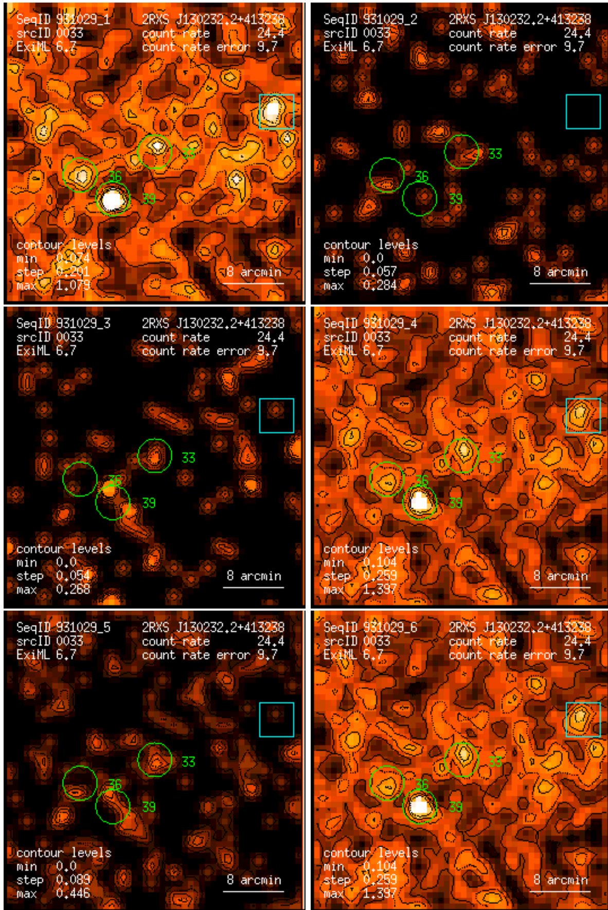
Figure 33: RASS 931029: detection 0033: band rate images, Gaussian filter: (1) PSPC channels 11 – 41, (2) 52 – 90, (3) 91 – 201, (4) 11 – 235, (5) 52 – 201, (6) 11 – 201. Broad band rates in counts/ks. Band rate contour levels in counts/ks/arcmin 2 .
