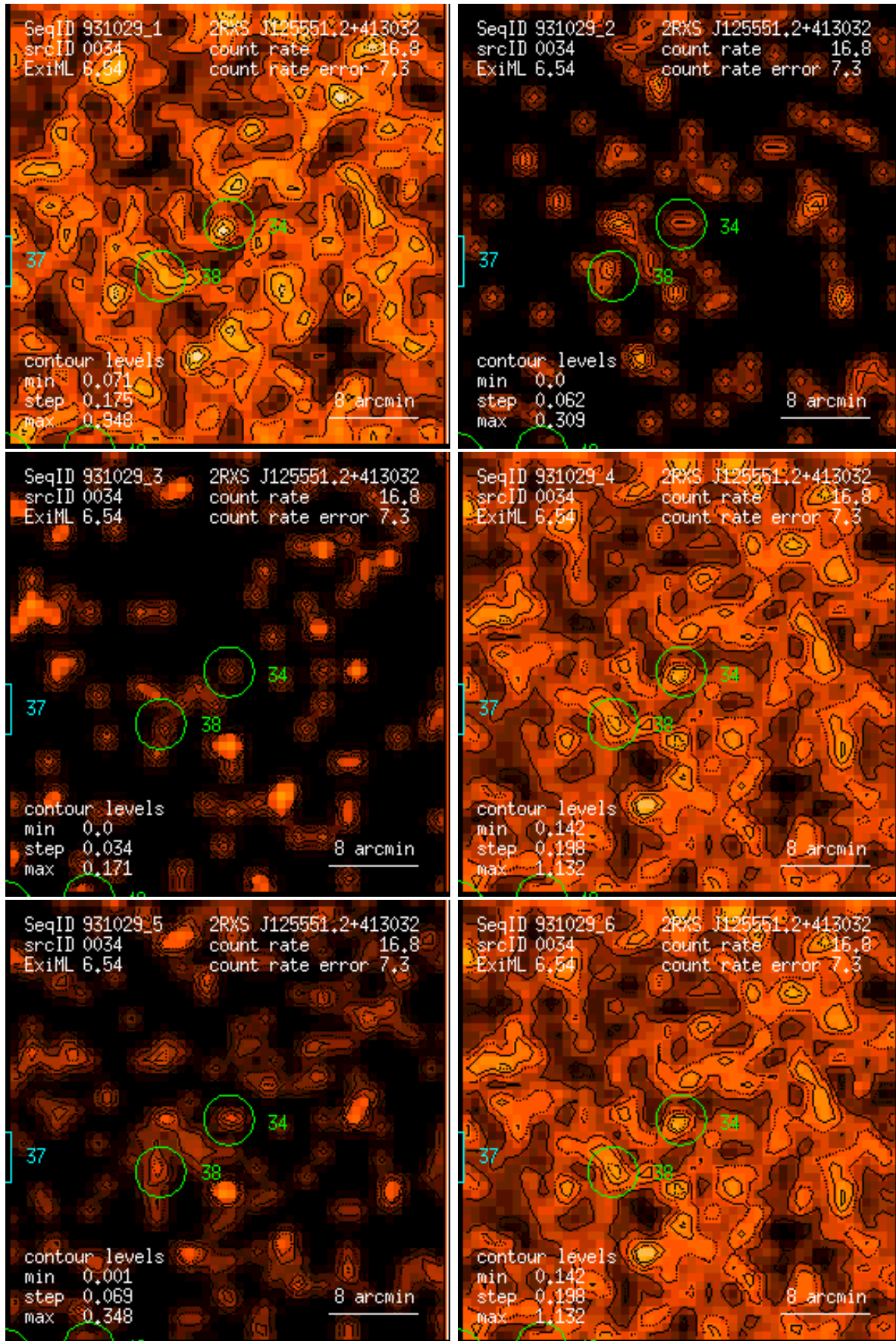
Figure 34: RASS 931029: detection 0034: band rate images, Gaussian filter: (1) PSPC channels 11 – 41, (2) 52 – 90, (3) 91 – 201, (4) 11 – 235, (5) 52 – 201, (6) 11 – 201. Broad band rates in counts/ks. Band rate contour levels in counts/ks/arcmin 2 .
