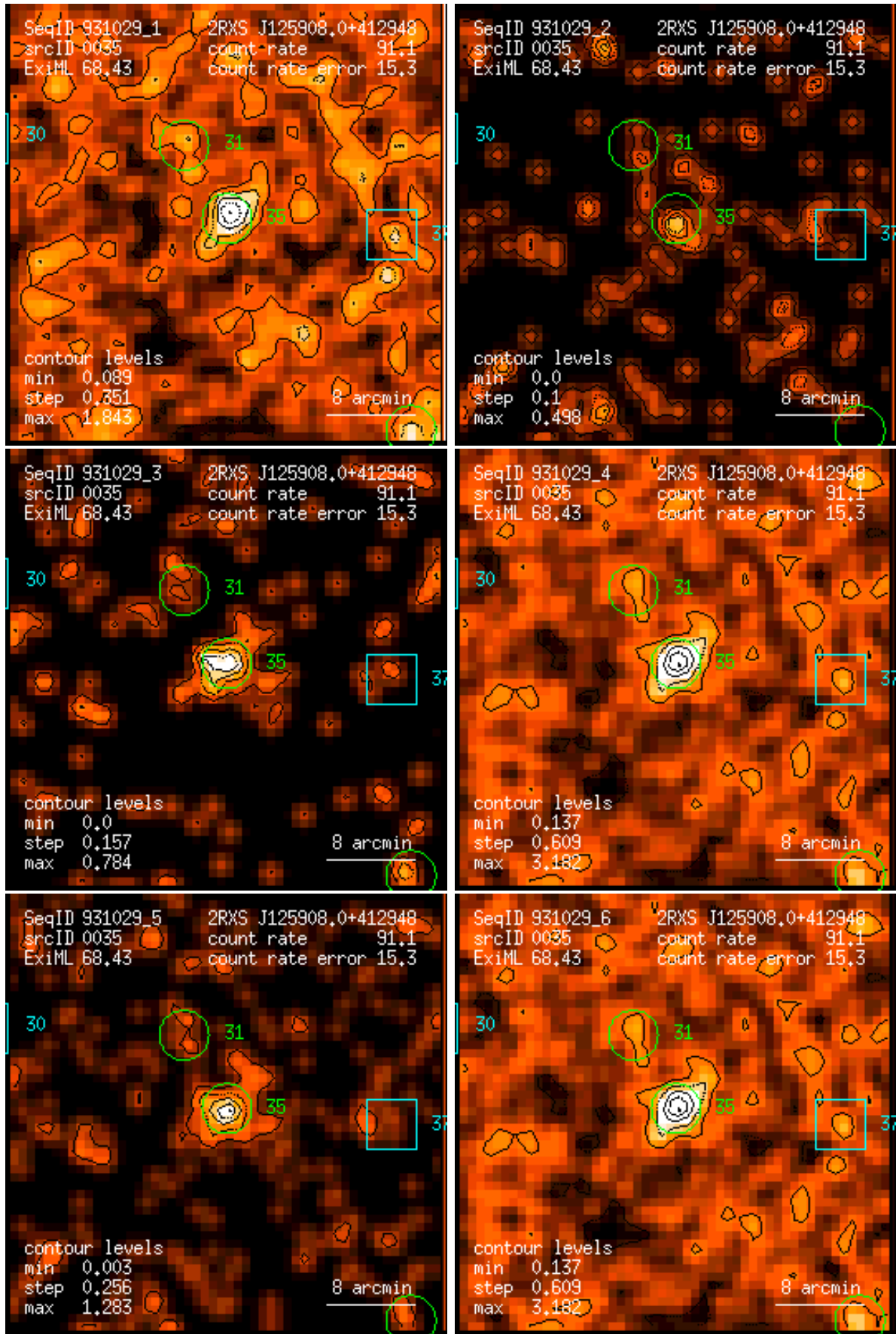
Figure 35: RASS 931029: detection 0035: band rate images, Gaussian filter: (1) PSPC channels 11 – 41, (2) 52 – 90, (3) 91 – 201, (4) 11 – 235, (5) 52 – 201, (6) 11 – 201. Broad band rates in counts/ks. Band rate contour levels in counts/ks/arcmin 2 .
