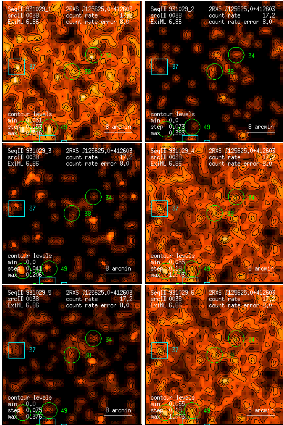
Figure 38: RASS 931029: detection 0038: band rate images, Gaussian filter: (1) PSPC channels 11 – 41, (2) 52 – 90, (3) 91 – 201, (4) 11 – 235, (5) 52 – 201, (6) 11 – 201. Broad band rates in counts/ks. Band rate contour levels in counts/ks/arcmin 2 .
