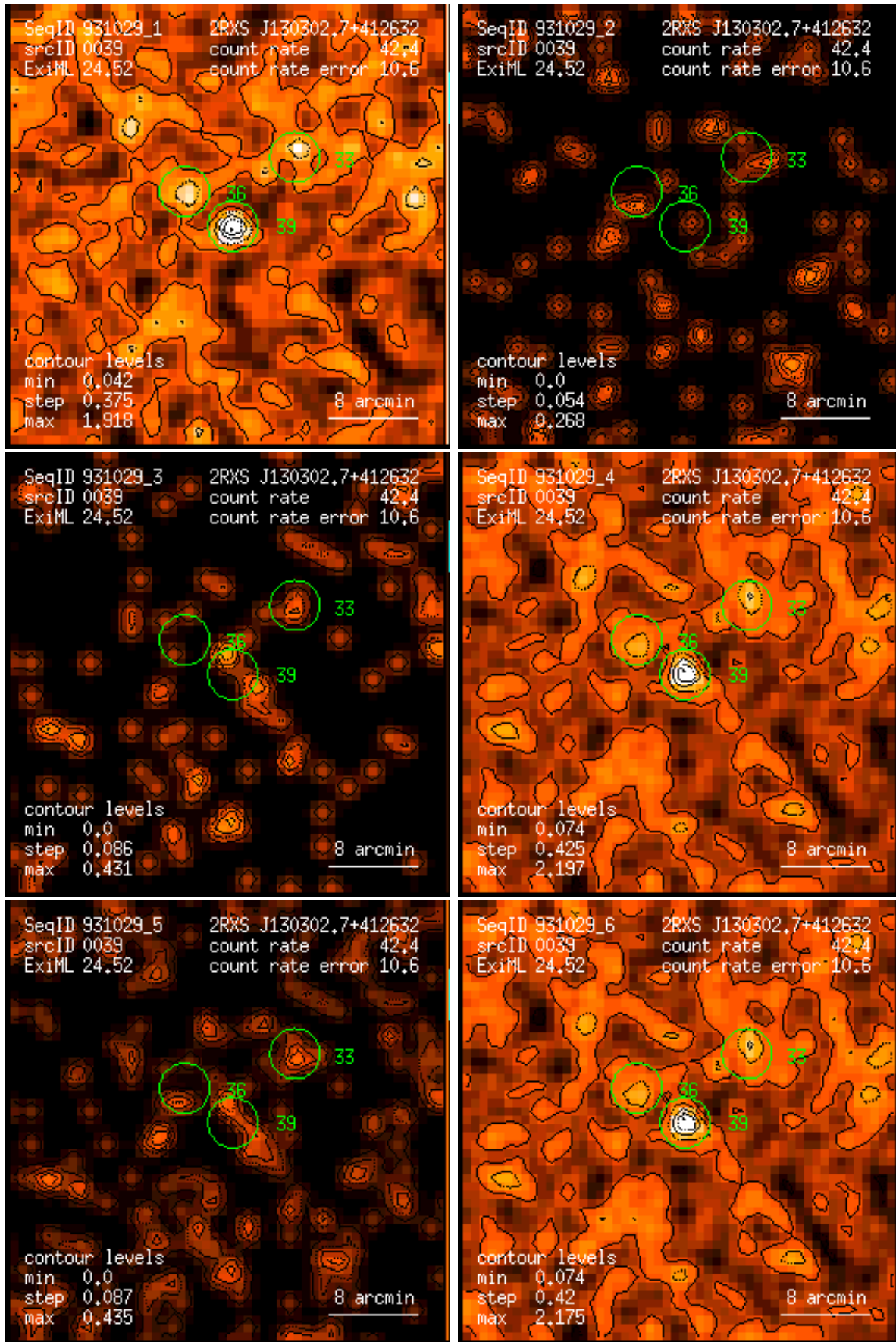
Figure 39: RASS 931029: detection 0039: band rate images, Gaussian filter: (1) PSPC channels 11 – 41, (2) 52 – 90, (3) 91 – 201, (4) 11 – 235, (5) 52 – 201, (6) 11 – 201. Broad band rates in counts/ks. Band rate contour levels in counts/ks/arcmin 2 .
