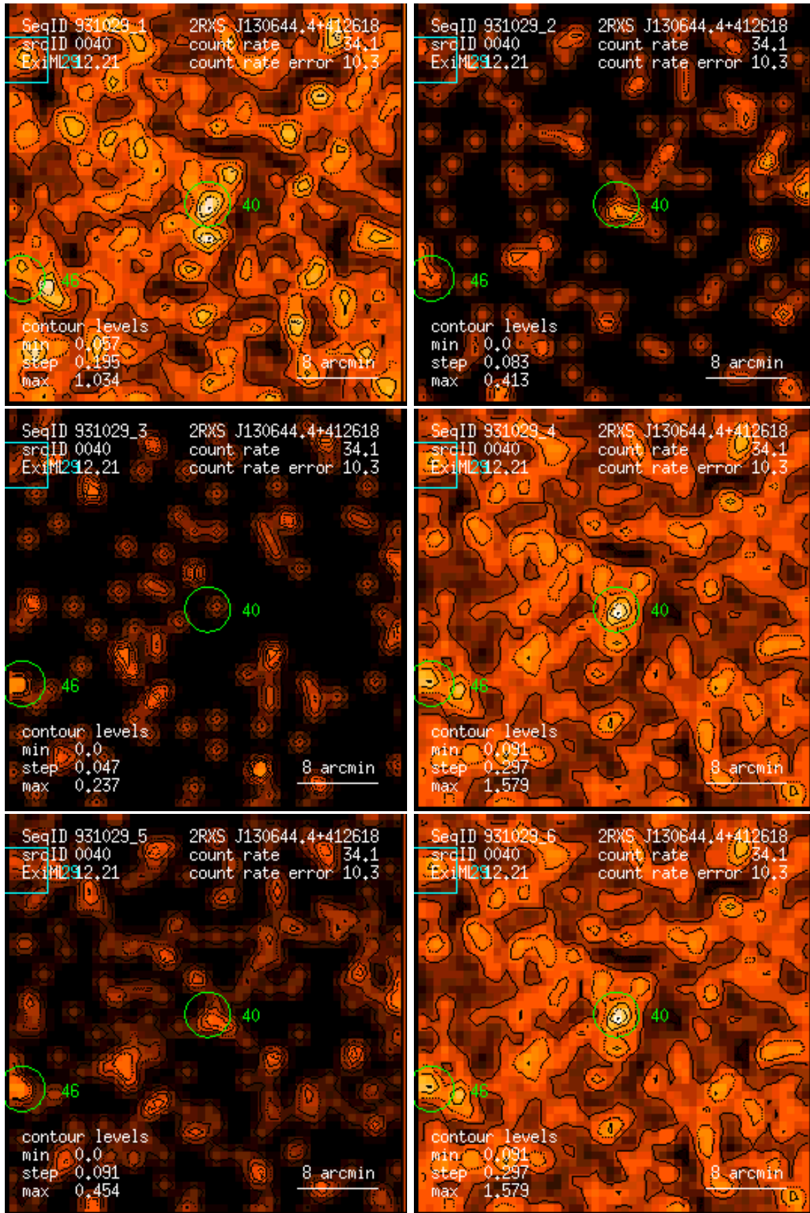
Figure 40: RASS 931029: detection 0040: band rate images, Gaussian filter: (1) PSPC channels 11 – 41, (2) 52 – 90, (3) 91 – 201, (4) 11 – 235, (5) 52 – 201, (6) 11 – 201. Broad band rates in counts/ks. Band rate contour levels in counts/ks/arcmin 2 .
