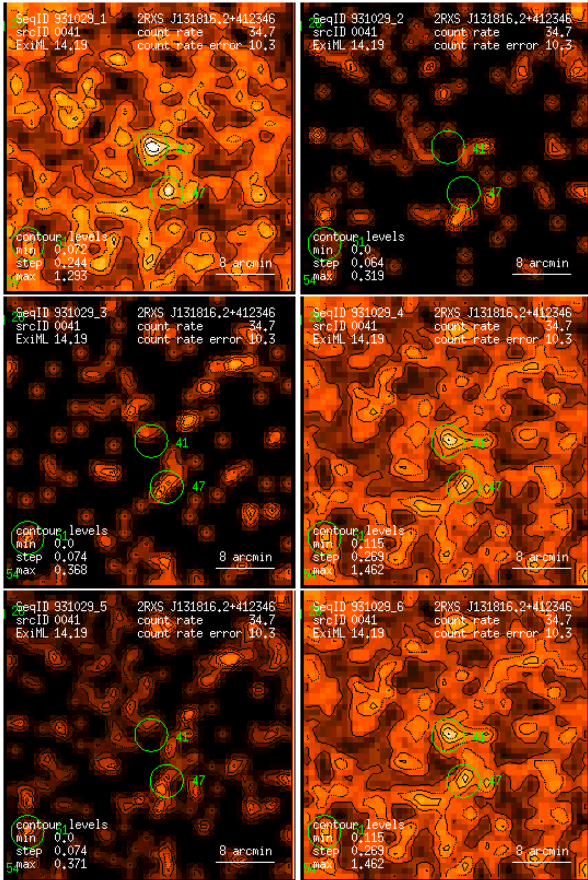
Figure 41: RASS 931029: detection 0041: band rate images, Gaussian filter: (1) PSPC channels 11 – 41, (2) 52 – 90, (3) 91 – 201, (4) 11 – 235, (5) 52 – 201, (6) 11 – 201. Broad band rates in counts/ks. Band rate contour levels in counts/ks/arcmin 2 .
