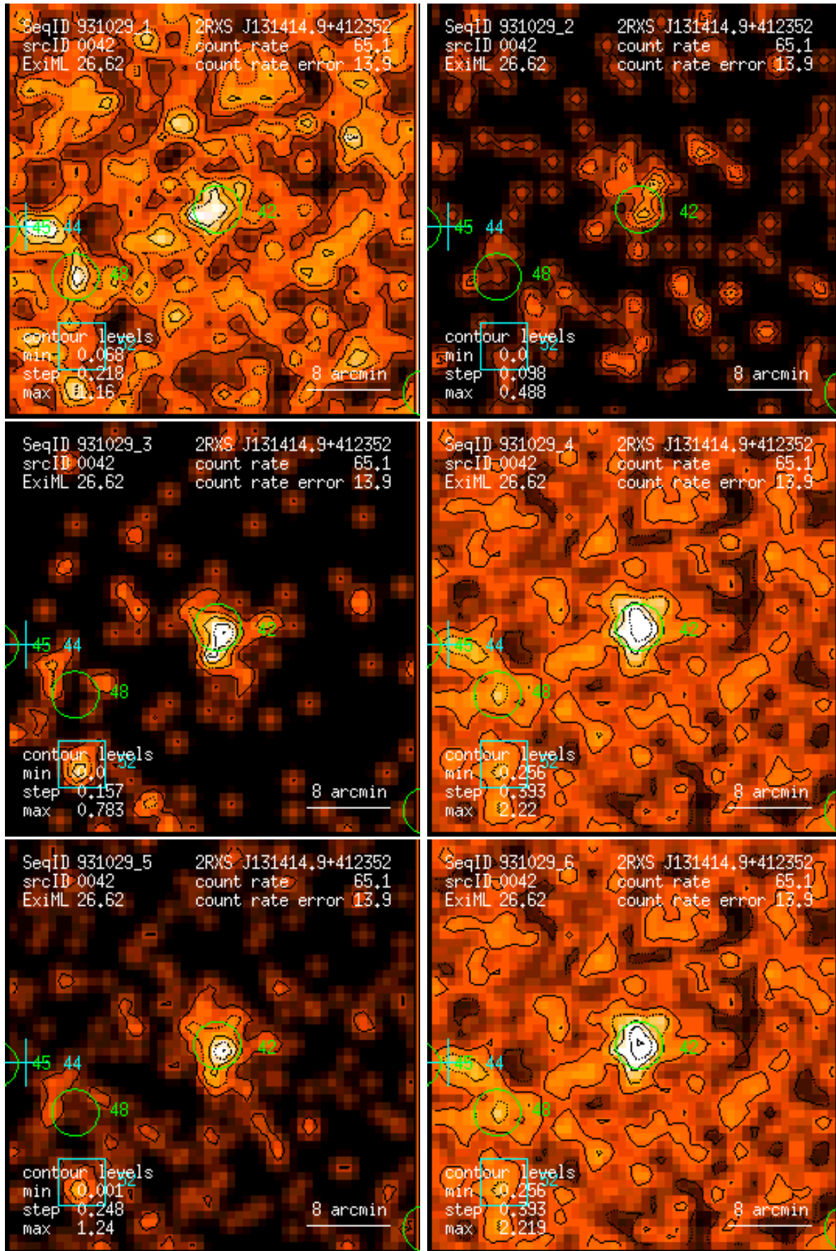
Figure 42: RASS 931029: detection 0042: band rate images, Gaussian filter: (1) PSPC channels 11 – 41, (2) 52 – 90, (3) 91 – 201, (4) 11 – 235, (5) 52 – 201, (6) 11 – 201. Broad band rates in counts/ks. Band rate contour levels in counts/ks/arcmin 2 .
