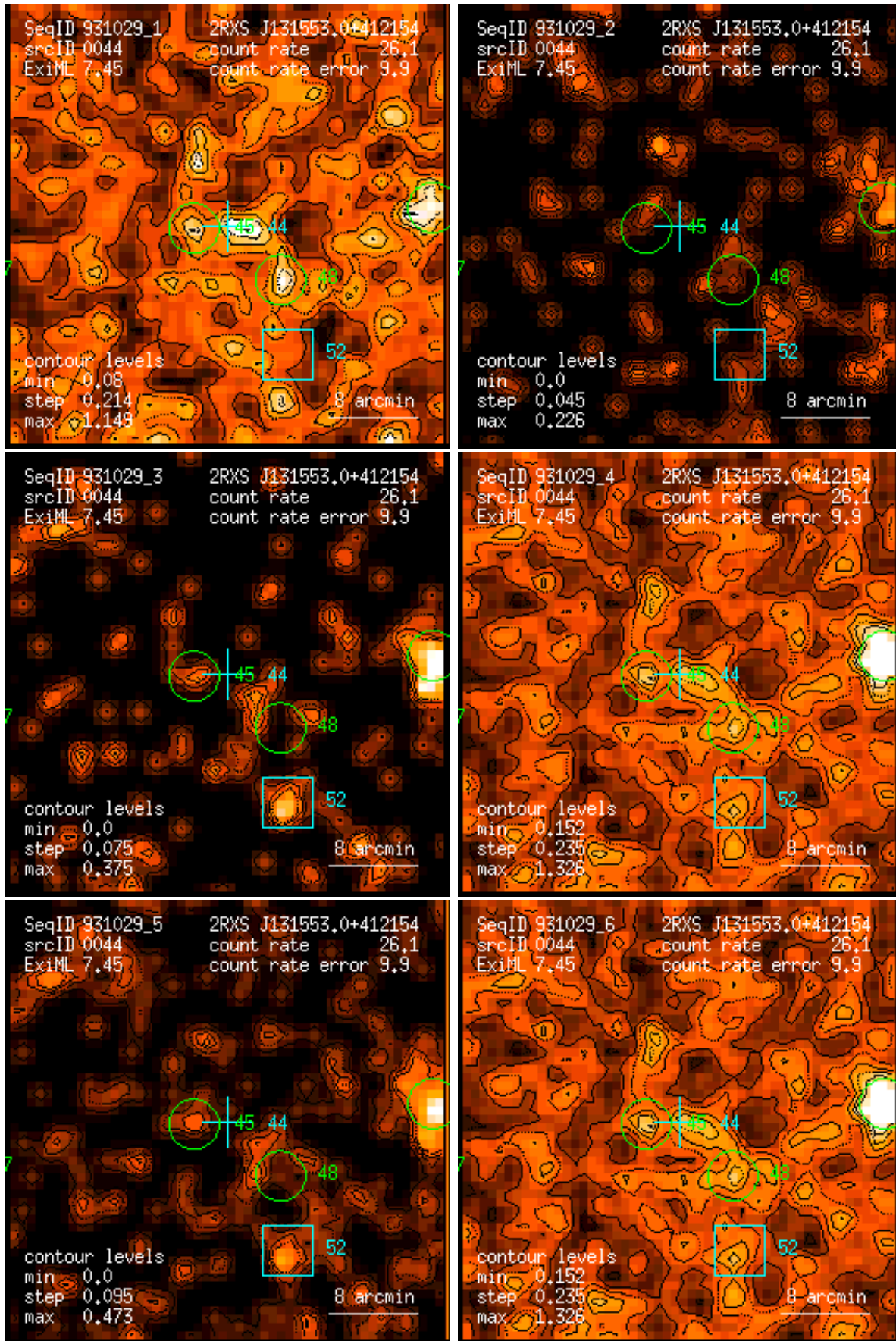
Figure 44: RASS 931029: detection 0044: band rate images, Gaussian filter: (1) PSPC channels 11 – 41, (2) 52 – 90, (3) 91 – 201, (4) 11 – 235, (5) 52 – 201, (6) 11 – 201. Broad band rates in counts/ks. Band rate contour levels in counts/ks/arcmin 2 .
